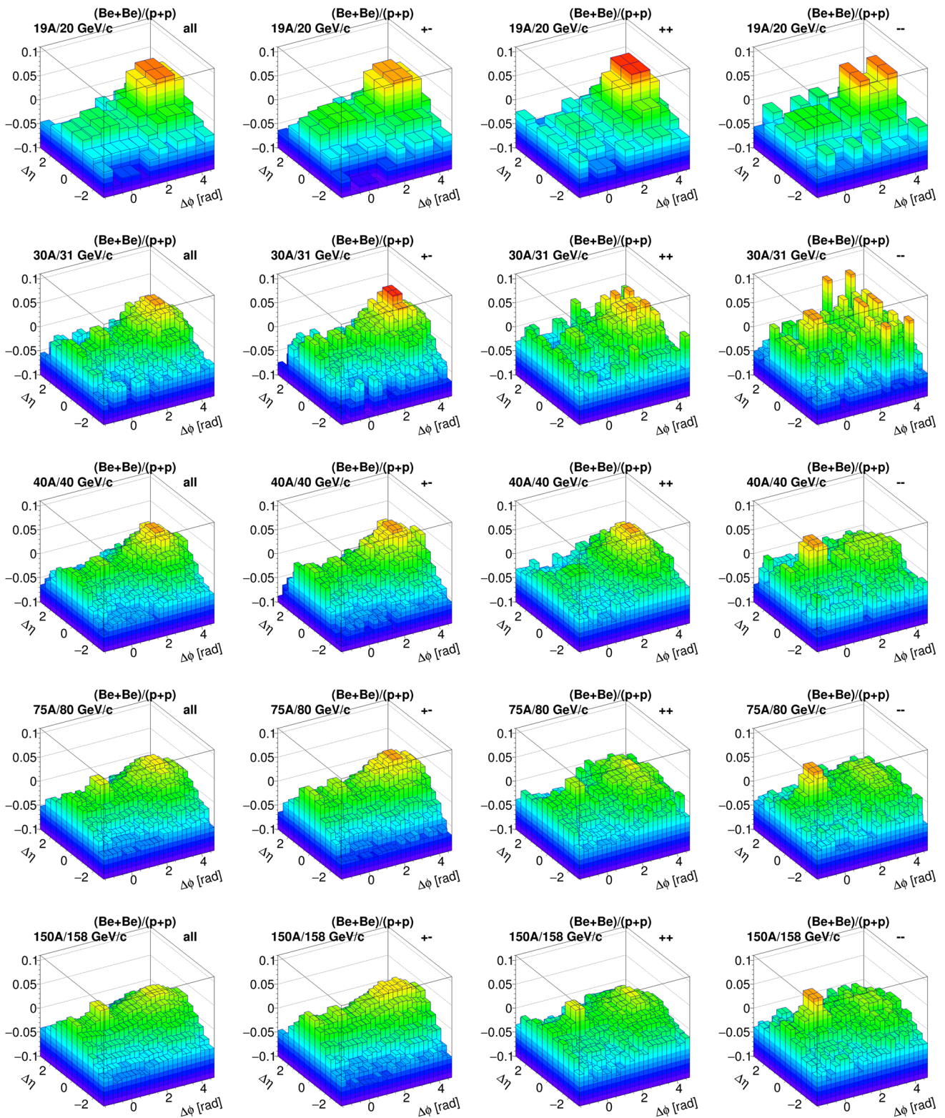
Fig. 11 Ratio R_{pp}^{\text{BeBe}} for all pair combinations and momenta (following formula Eq. 4). Each row shows different beam momentum (beam momentum increases downwards). Every column presents results for
