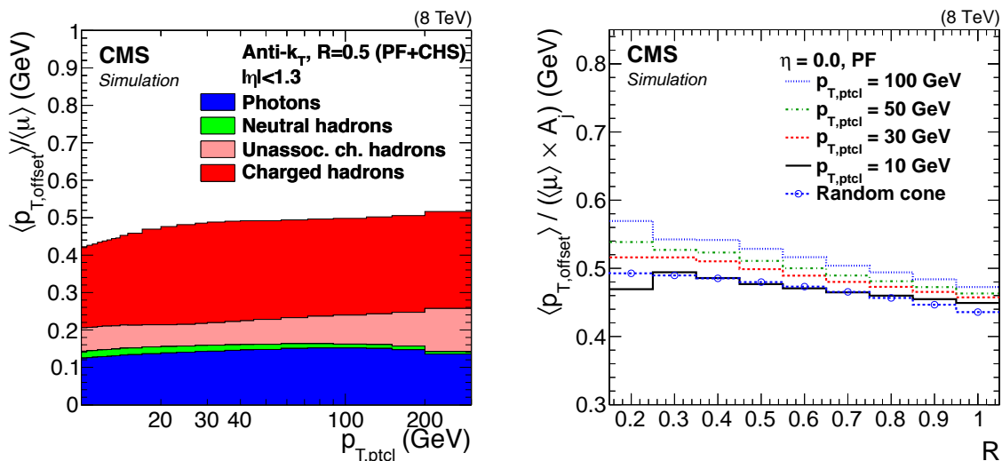
Figure 6. Simulated particle-level offset versus p_T separately for each type of PF candidate (left). Average p_T offset density versus jet distance parameter R for various p_{T,ptcl} compared to a random-cone offset density versus cone radius (right). The jet or cone area A_j corresponds to \pi R^2 .
