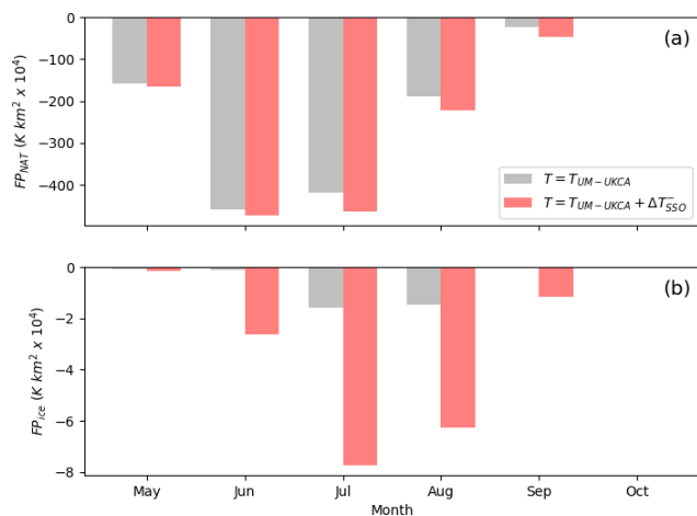
Figure 7. Histograms showing the monthly mean formation potential ( \times 10^4 K km 2 ; see (1) for definition) for PSCs made from (a) NAT and (b) ice particles during each individual month from May to October at an altitude of 20.4 km for the perturbation run (red) and the control run (grey), i.e. for T equal to either T_{UM-UKCA} + \Delta T_{SSO}^- (perturbation run with the parameterisation scheme on) or T_{UM-UKCA} (control run with the parameterisation scheme off). Note that the results are computed within the box indicated in Fig. 1.
