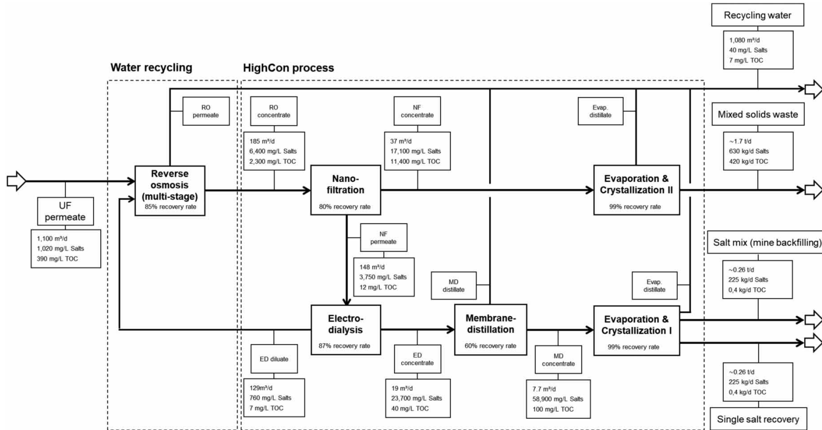
Figure 11 | Simplified process flow sheet for the full-scale water recycling and HighCon concentrate treatment designed for an inflow of 1,100 m³/d MBR UF permeate from coffee production wastewater treatment.
