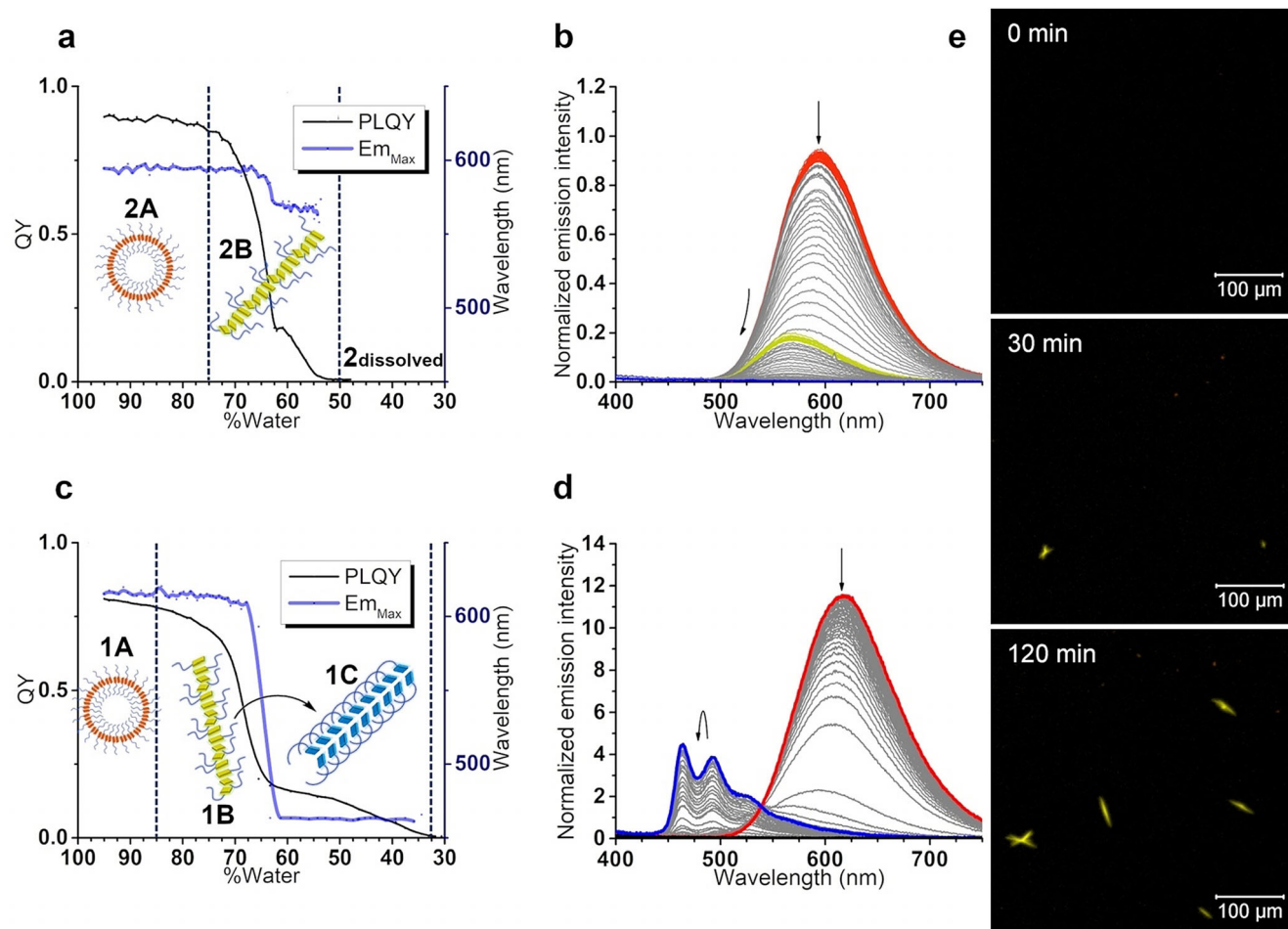
Figure 2. a) Depolymerization profile of compound 2 ( c = 5 \times 10^{-5} M) showing the PLQY and emission maximum, as a function of the ratio water:dioxane in the system. b) Spectra profile of the depolymerization experiment for 2 , from the starting orange emissive aggregates at high water content (red line spectra) to a second class of yellow-emissive structures (yellow line) below 70% water content, to the molecularly dissolved state when the water content is below 50% (blue line), \lambda_{\text{ex}} = 313 nm. c) Depolymerization profile of compound 1 ( c = 1 \times 10^{-4} M) showing the PLQY and emission maximum, as a function of the % of water in the system. d) Spectra profile of the depolymerization experiment for 1 , the starting orange-emissive aggregates at high water content (red line spectra) to the blue-emitting nanoribbons (blue line) below 70% water content to the molecularly dissolved state when the water content is below 30%, \lambda_{\text{ex}} = 313 nm. Spectra profile of the depolymerization experiment for 1 adapted, with permission of Springer Nature, from ref. [12]. e) Snapshots taken from Supplementary Movie 1 showing the time-dependent evolution of the yellow assemblies ( 2B ) by confocal microscopy at 65% water content ( \lambda_{\text{ex}} = 405 nm) (more information is provided in the SI).
