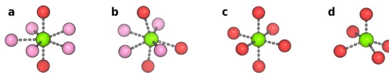
Figure 5. Different coordination states of Mg 2+ , colored in green, in the presence (a,b) and absence (c,d) of 18-crown-6. Oxygen atoms belonging to the 18-crown-6 ring are colored in pink; those belonging to TFSI - in red.
