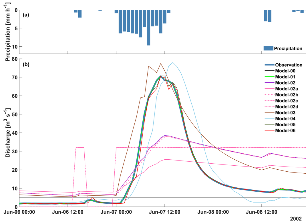
Figure 3. (a) Observed precipitation at Ebnet. (b) Observed discharge at gauge Hoher Steg and simulations thereof by Model-00 to Model-06 for a rainfall-runoff event in June 2002.
