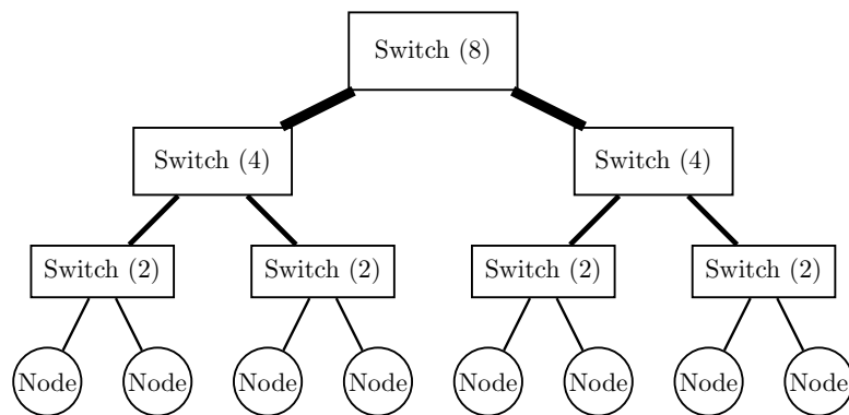
Figure 2.5: Fat-Tree network with 8 nodes.
