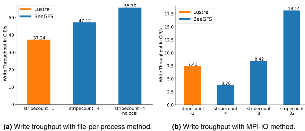
Figure 4.6: Different write throughput, based on implementation on file system configuration.
