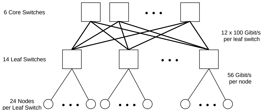
Figure 3.2: The small island consists of 6 core switches and 14 leaf switches. Each leaf switch has 24 nodes with 56 Gbit/s and 2x100 Gbit/s links to each core switch.
