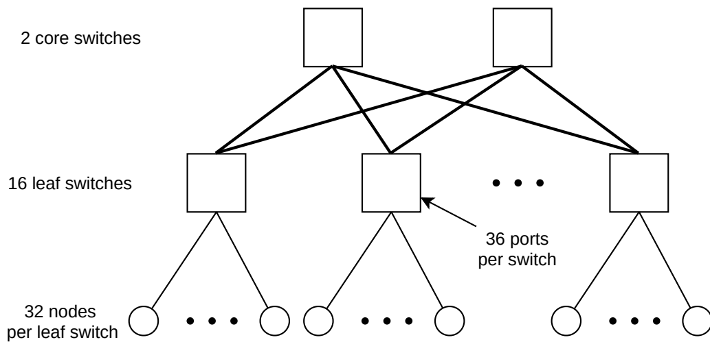
Figure 2.8: A CBB 1:8 blocking topology with 512 nodes.
