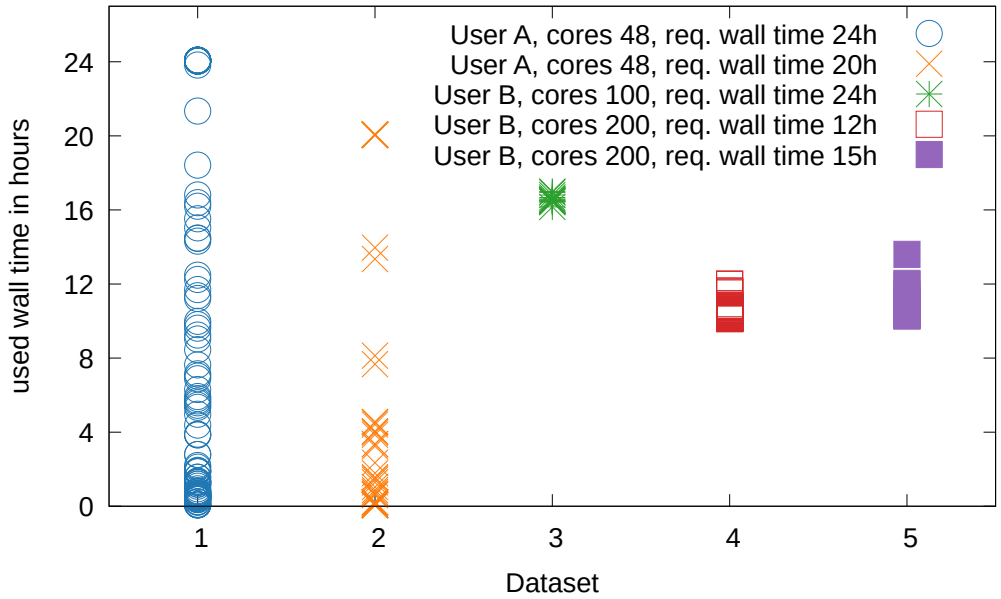
Figure 5.6: Real used wall time categorised by user, request wall time and core count. Category 1 and 2 shows a huge variance in the used wall time, while the other categories has a small variance.
