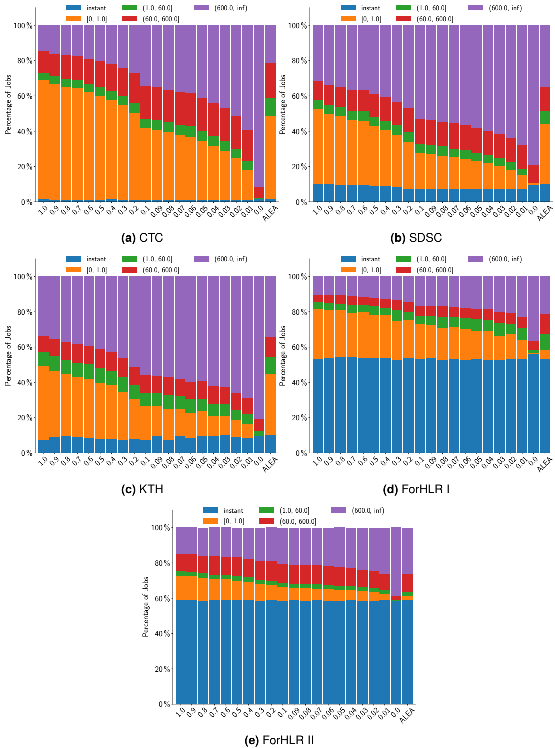
Figure 5.13: First Come First Serve (FCFS) algorithm. Job distributions according to the T_{NAP} class for all used workloads. X-axis: shows different \lambda values. Blue color denotes instant jobs, orange means job having T_{NAP} \leq 1 s, green denotes jobs with 1 \text{ s} < T_{NAP} \leq 60 s, red jobs with 60 \text{ s} < T_{NAP} \leq 600 s, and purple denotes long-term predictions ( 600 \text{ s} < T_{NAP} ).
