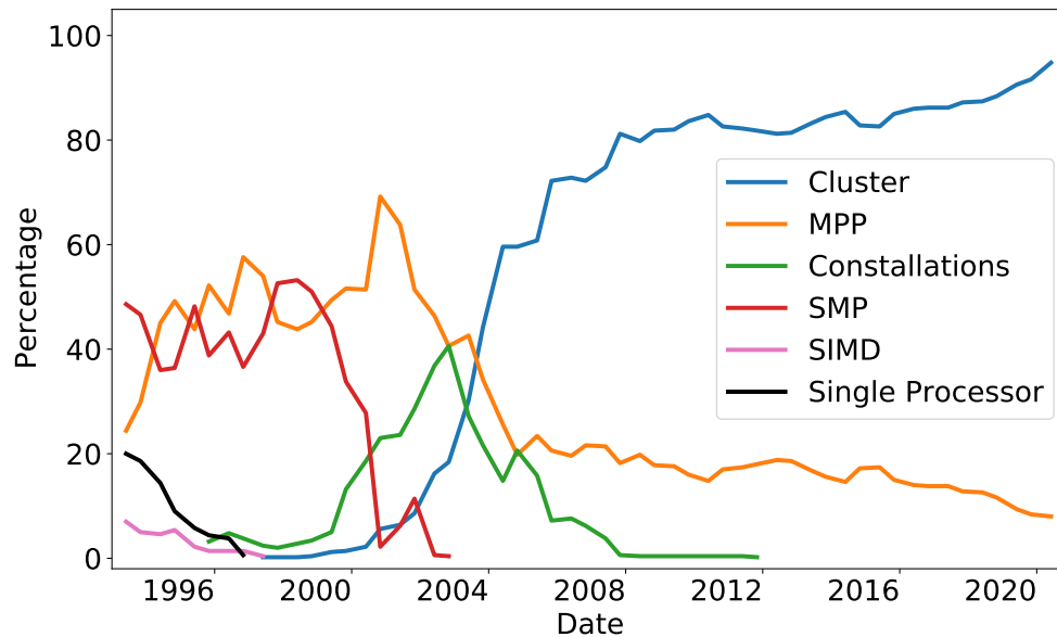
Figure 2.1: Design concepts change within the TOP 500 List. Data Source: www.top500.org
