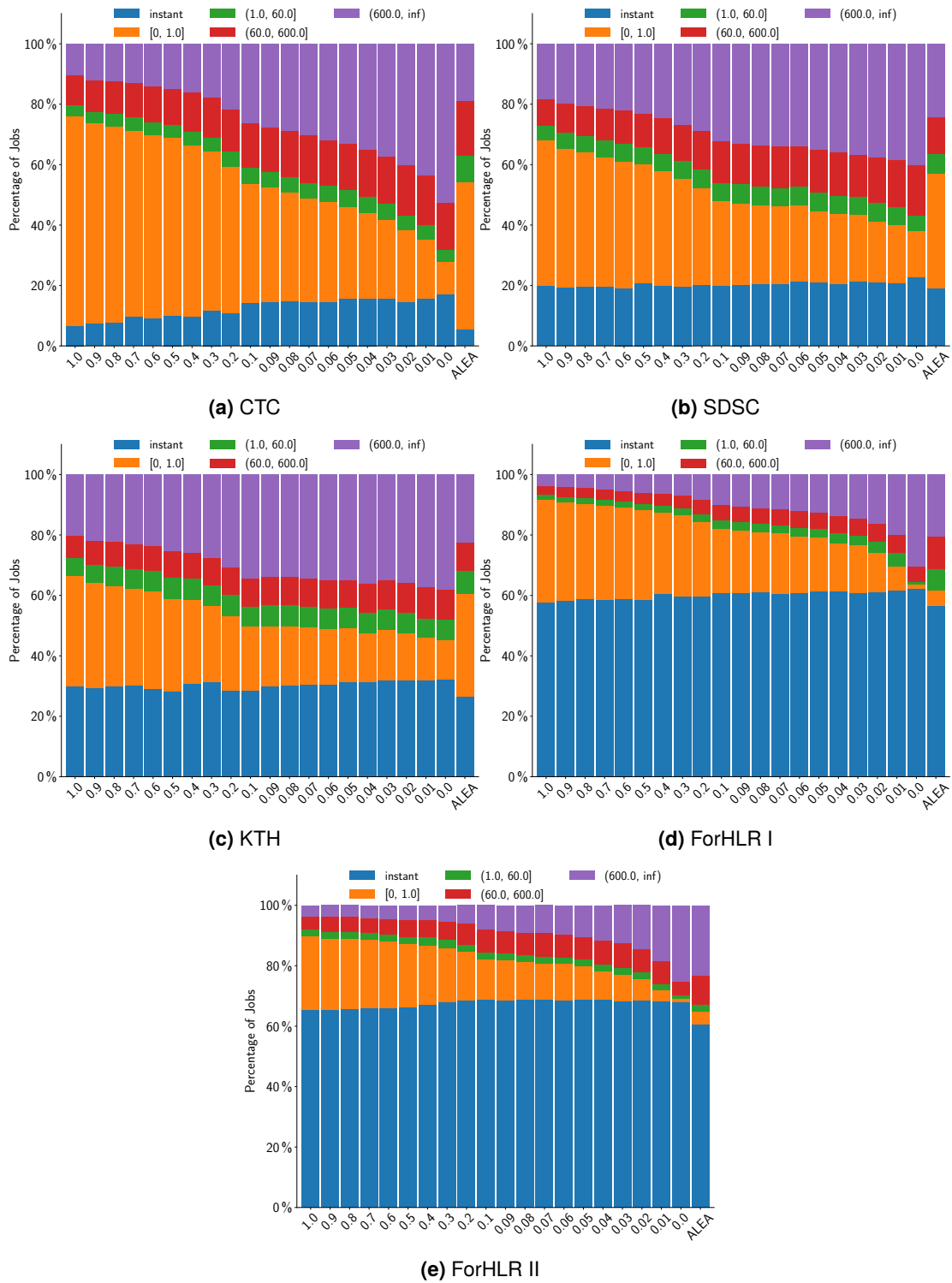
Figure 5.12: Conservative + Back-fill algorithm. Job distributions according to the T_{NAP} class for all used workloads. X-axis: shows different \lambda values. Blue color denotes instant jobs, orange means job having T_{NAP} \leq 1 s, green denotes jobs with 1 \text{ s} < T_{NAP} \leq 60 s, red jobs with 60 \text{ s} < T_{NAP} \leq 600 s, and purple denotes long-term predictions ( 600 \text{ s} < T_{NAP} ).
