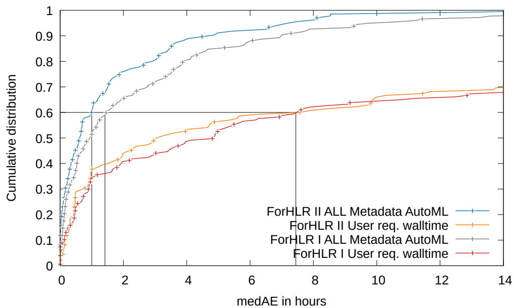
Figure 5.11: Comparison of medAE for ForHLR I+II. X-axis: Median absolute error in hours, Y-axis cumulative distribution.
