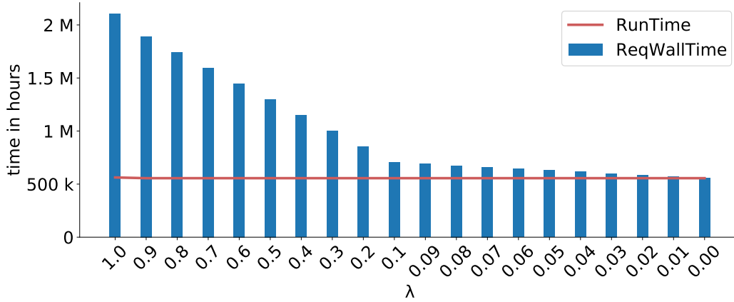
Figure 5.8: ForHLR II workload with improved estimates. Y-axis shows the sum requested and used hours.
