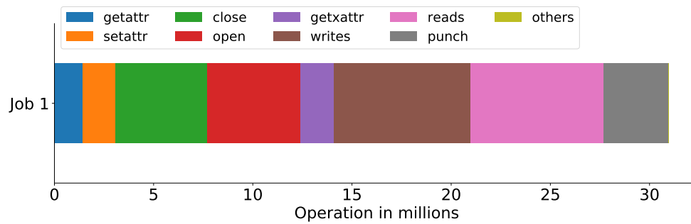
Figure 4.11: Total I/O operation created for one generation within approx. 20 min.
