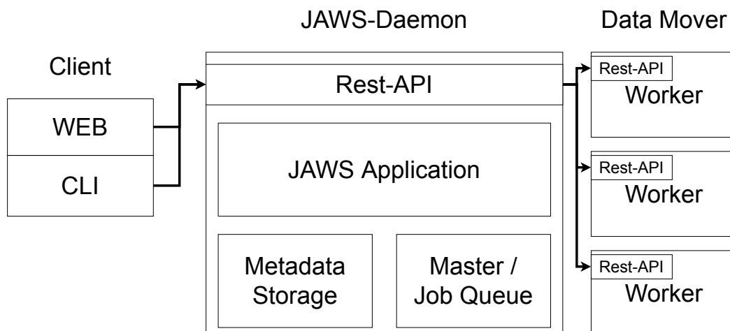
Figure 6.6: Design of the JAWS framework. Clients (Web/CLI) access the main daemon via REST API. JAWS Daemon communicates via REST API with distributed worker.
