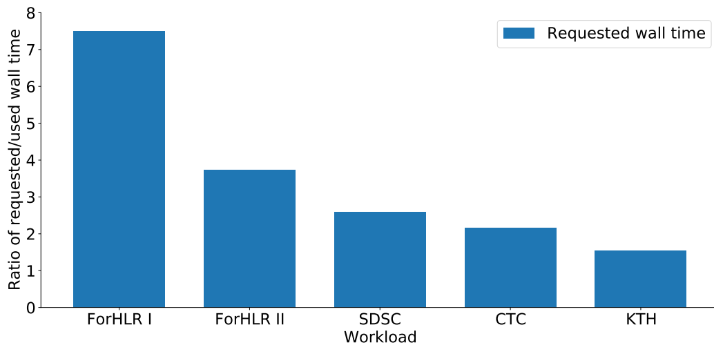
Figure 5.5: Ratio of requested and used wall time compared for different historic workloads..
