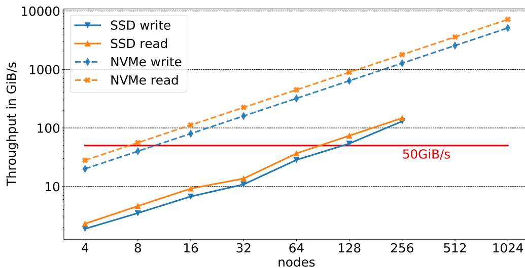
Figure 4.3: Measured read/write throughput (solid) and extrapolated (dashed) with announced speeds of NVMe-SSDs [112]. Horizontal red line shows the performance of the fastest PFS attached to ForHLR II.
