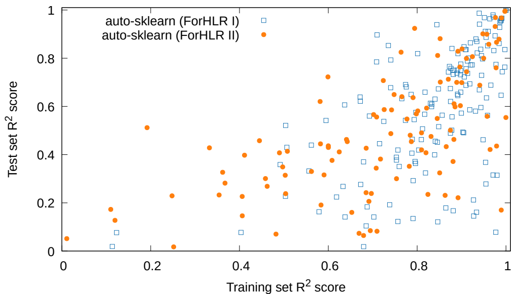
Figure 5.7: The x-axis shows the R^2 score on training samples and the y-axis shows R^2 score on test samples for the work load files from ForHLR I+II. Models trained with automatic Machine learning for 20 min each model.
