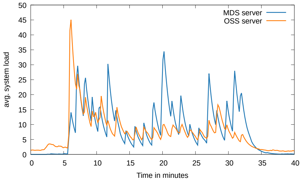
Figure 4.8: Load generated by the OpenFOAM use case. Minutes 0–5 and 35–40 show usual load during normal operation.
