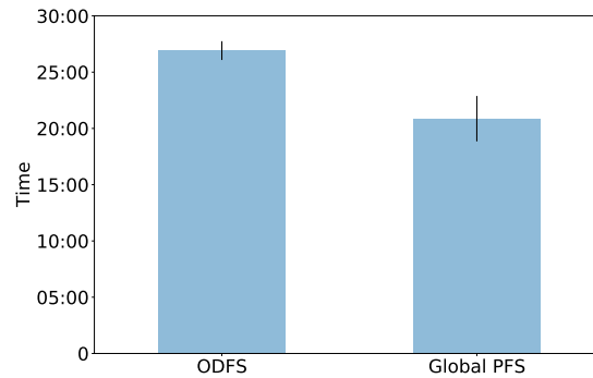
Figure 4.12: Average run time for one generation.
