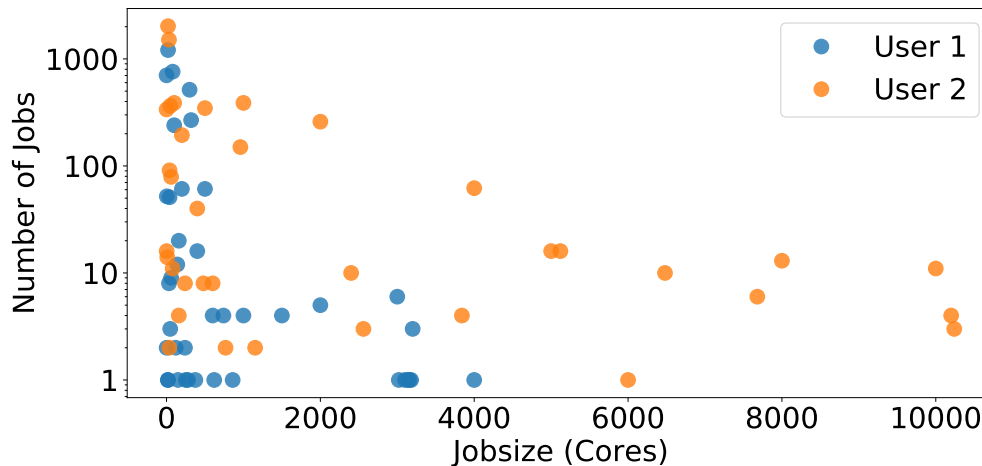
Figure 6.5: Distribution of jobsizes for two scientists based on their HPC usage at SCC. Details can be taken from Table A.1.
