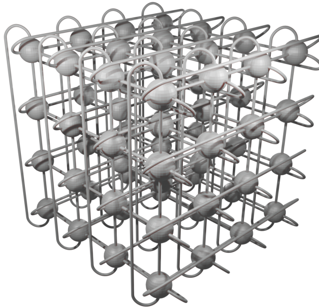
Figure 2.6: Three-dimensional torus interconnection of 4 \times 4 \times 4 nodes. The connection in each dimension has a loop from the first to the last node. Artwork by Marco Berghoff [58].
