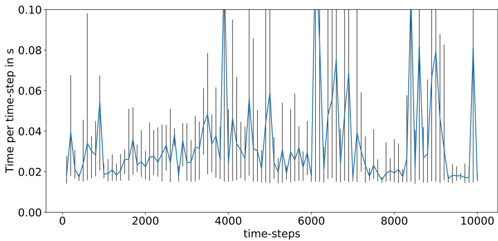
(b) NASTJA using global file system
