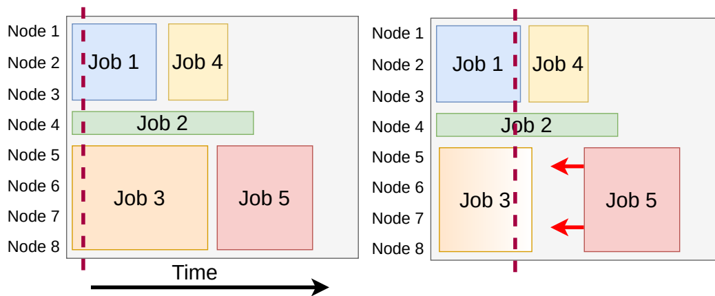
Figure 5.4: Job 3 finishes early. Job 5 jumps forward. Same nodes but earlier start time.
