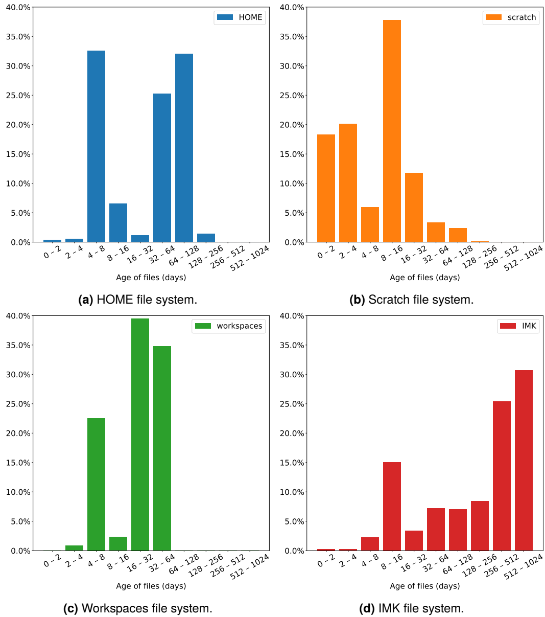
Figure 6.4: Age of files since creation on different file systems.
