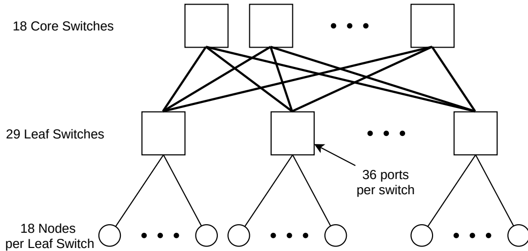
Figure 2.7: A CBB fully non-blocking topology with 512 nodes. Note, the last leaf switch has only 8 nodes.
