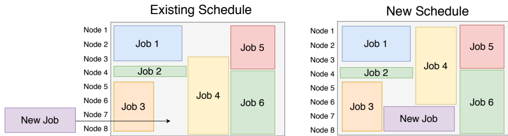
Figure 5.2: Re-scheduling of jobs to other nodes so that a new job can be back-filled.
