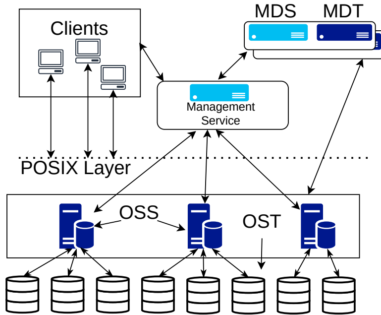
Figure 2.13: Simple overview of BeeGFS file system components. Storage services consist of Object Storage Server (OSS) and Object Storage Targets (OST). Clients access the storage services via a POSIX Layer. BeeGFS can have multiple Metadata Server (MDS) and Metadata Target (MDT). A central management service serves as registry for clients and servers.
