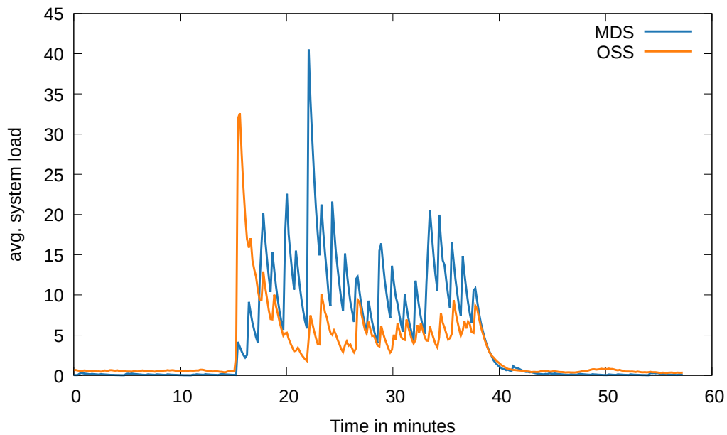
Figure 3.3: Average UNIX load caused on the Lustre file system during a simulation run of 25 min. Minutes 0–15 and 40–60 show the usual load on the Lustre file system.
