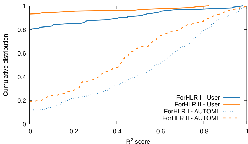
Figure 5.9: X-axis R^2 score on test samples, Y-axis cumulative distribution for ForHLR I+II. Solid line show R^2 for user estimates. Dashed lines show R^2 for AutoML trained models.
