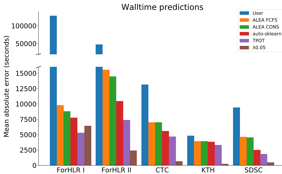
Figure 5.14: The mean absolute error (MAE) for different predictions on different workloads.
