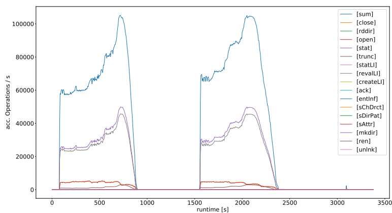
Figure A.1: IOPS over time for two generation. (Swarm-based meta-heuristic)
