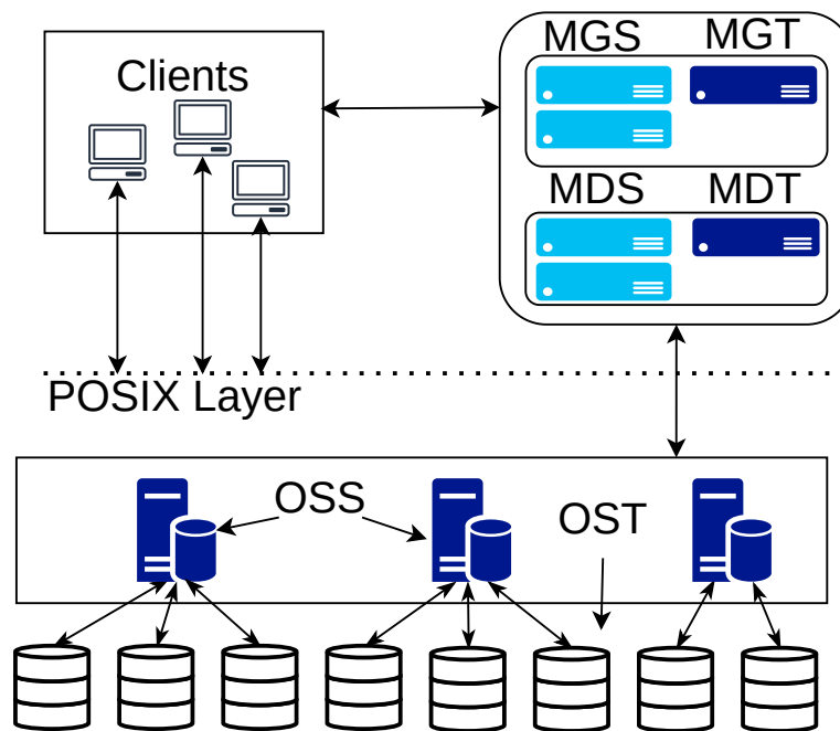
Figure 2.14: Simple overview of Luster file system components. Storage services consist of Object Storage Server (OSS) and Object Storage Targets (OST). Clients access the storage services via a POSIX Layer. Luster can have multiple Metadata Server (MDS) and Metadata Target (MDT). Multiple Luster Management Services (MGS) serves as a management service. Servers and clients connect to a MGS on startup to retrieve the configuration for the Luster file system.
