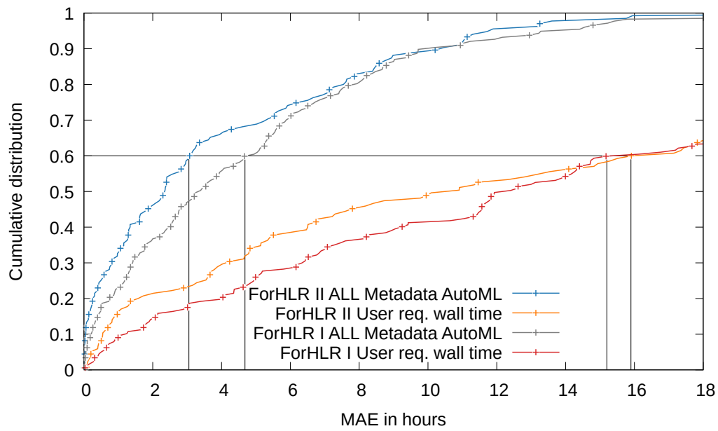
Figure 5.10: Comparison of MAE for ForHLR I+II. X-axis: mean absolute error in hours, Y-axis cumulative distribution.
