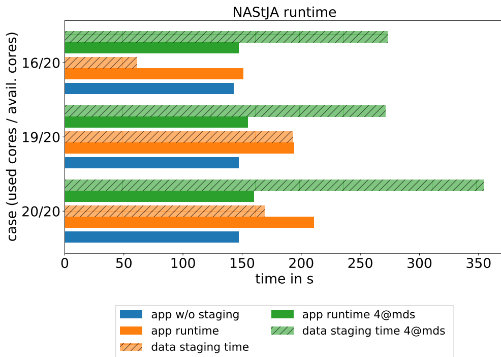
Figure 4.14: Total execution time (NASTJA) for application w/o data staging.
