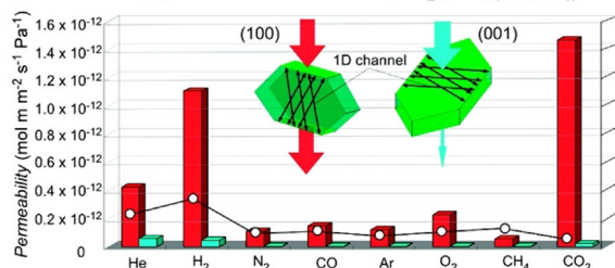
Figure 7. A) ZIF-8 single crystal mounted on a metal plate with a 100 μm hole in it. Reprinted from Chen et al. [25] with permission from Elsevier ©2019. B) Measuring anisotropic gas permeation through [Cu 2 (bza) 4 (pyz)] n with 1D channels. The channels in the (100) direction are free for gas transport, no gas permeation occurs in the (001) direction. Reprinted from Takamizawa et al. [65] with permission from the American Chemical Society ©2010.
