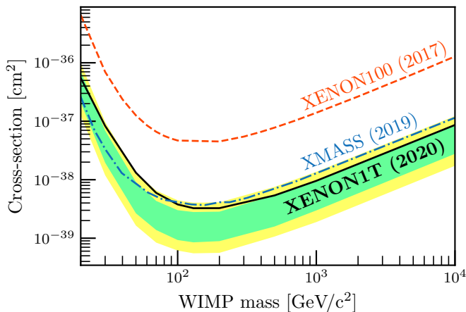
FIG. 4. Upper limit, at 90% CL, on the cross-section for inelastic scattering of WIMPs off xenon nuclei. The expected range at 1\sigma and 2\sigma is shown in green and yellow, respectively. Our result is compared to upper limits obtained by the XMASS collaboration [47] (blue dot-dashed line) and XENON100 [48] (orange dashed line).
