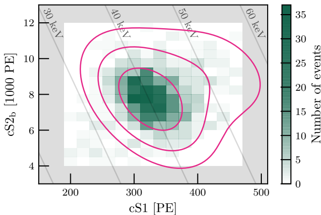
FIG. 1. Model for inelastic scattering of neutrons (pink 1\sigma , 2\sigma and 3\sigma contours) compared to calibration data with the neutron generator deployed. The density of calibration data is represented by the shading inside the 2\sigma contour, while outside individual events in the calibration data are shown as green dots. The white unshaded region indicates the region in which the fit is performed. Energy contours are shown as grey lines.
