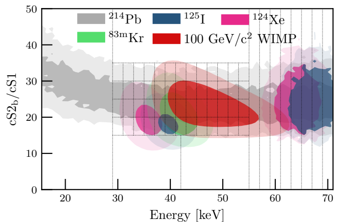
FIG. 2. Region of interest showing the four nominal background models: ^{214}\text{Pb} in grey, ^{83\text{m}}\text{Kr} in green, ^{124}\text{Xe} in pink and ^{125}\text{I} in blue; and the expected signal for a 100\text{ GeV}/c^2 WIMP in red. In each case the darker and lighter shading shows the 1\sigma and 2\sigma region, respectively. The cS2_b/cS1 distribution for ^{214}\text{Pb} is used to visualise the 2\nu\text{ECEC-KK} and EC-K peaks, which are only modelled in energy. The dotted lines indicate the boundaries of the bins used to perform the likelihood fit.
