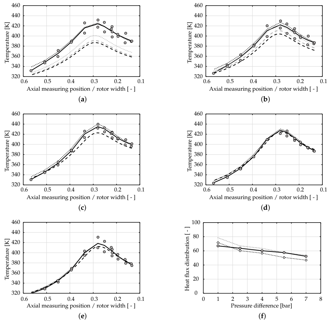
Figure 7. (a–e): Measuring points from experiment (○), Fit of the measured values from experiment (—), FE-Analysis (⋯⋯), CFD with \alpha_b = adjusted (---), CFD with \alpha_b = 100 \text{ W}/(\text{m}^2 \text{ K}) (-·-·-), CFD with \alpha_b = 1000 \text{ W}/(\text{m}^2 \text{ K}) (---); (f): Heat flux distribution under variation of the pressure difference, Experiment (◊), CFD (◻), CFD (target) (⋯⋯), (a) \Delta p = 1.0 bar, (b) \Delta p = 2.5 bar, (c) \Delta p = 4.0 bar, (d) \Delta p = 5.5 bar, (e) \Delta p = 7.0 bar.
