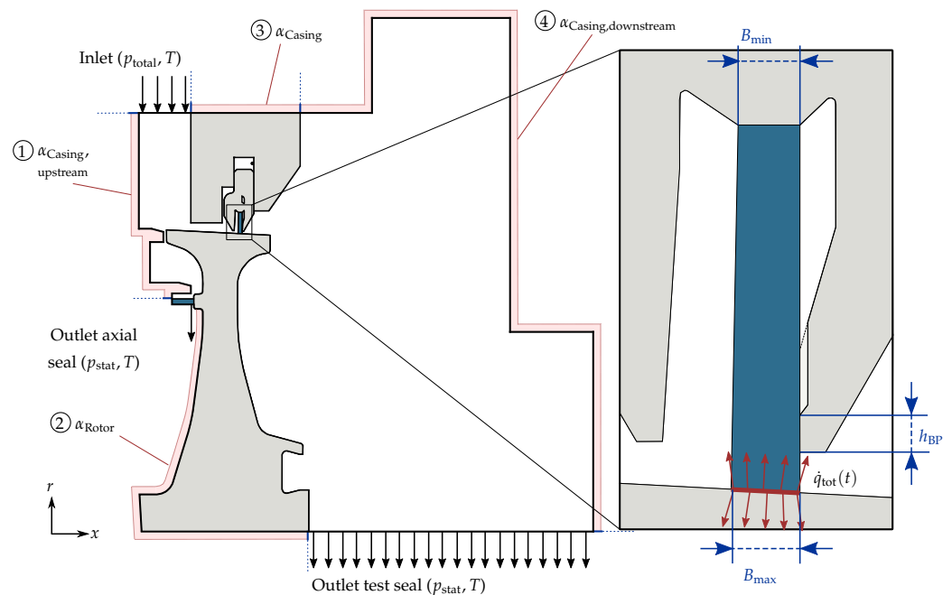
Figure 1. Computational domain of the numerical model; Fluid (□), Solid (▣), Porous media (■).
