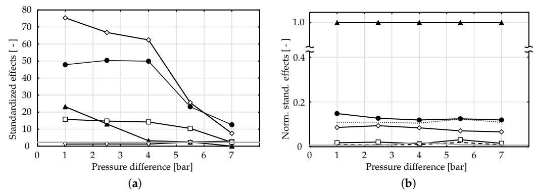
Figure 12. Standardized effects over variation of the pressure difference, significance level \alpha = 0.05 , \lambda_{\text{Rotor}} (●), \alpha_b (◆), A (▲), \lambda_{\text{Rotor}} \times \lambda_{\text{Rotor}} (▼), \alpha_b \times \alpha_b (■), A \times A (⋯), \lambda_{\text{Rotor}} \times A (—), Reference line (—), (a): Response variable: Heat flux distribution, (b): Response variable: Max. temperature in rubbing contact.
