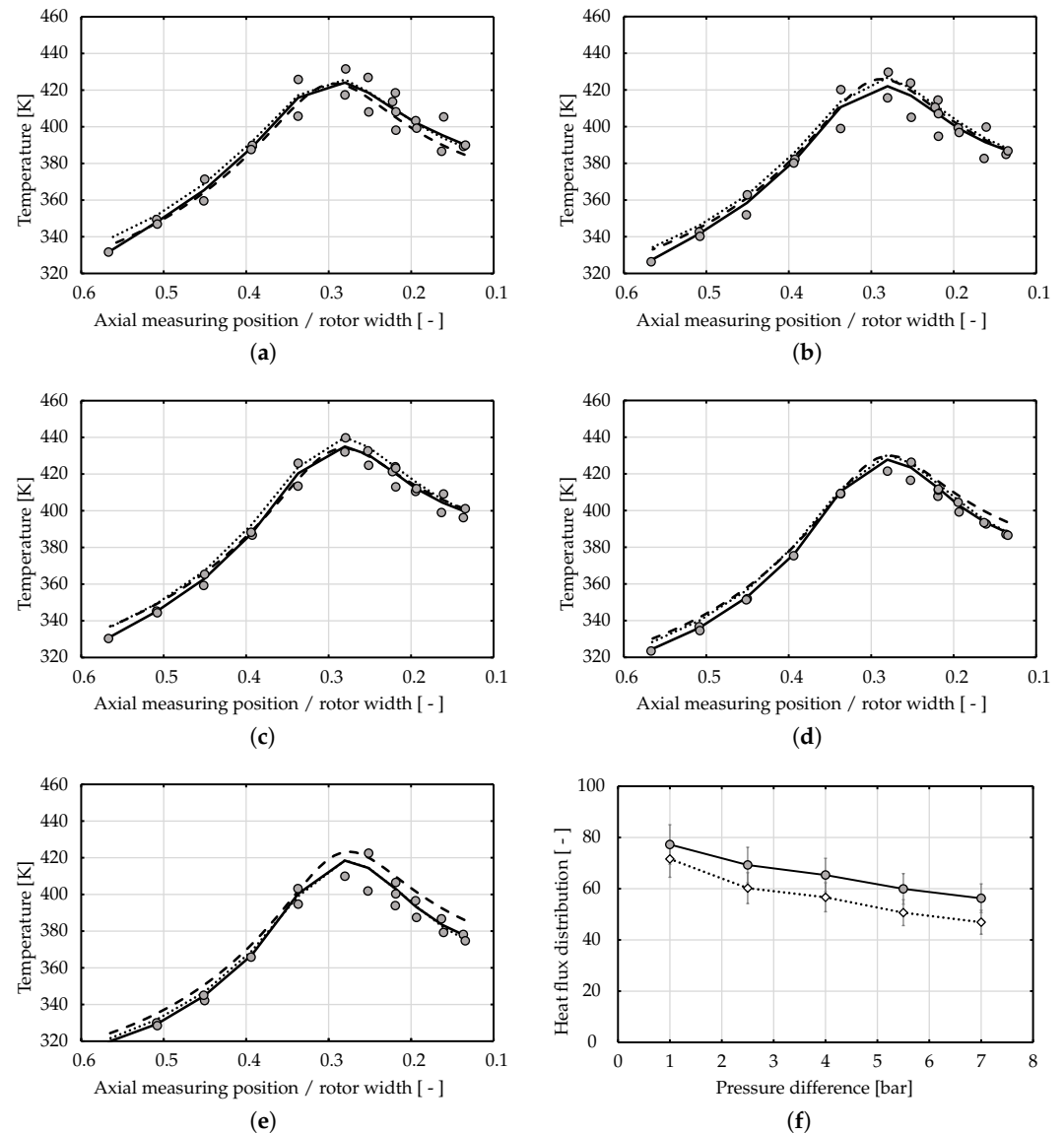
Figure 13. (a–e): Measuring points from experiment (○), Fit of the measured values from experiment (—), FE-Analysis (⋯⋯), CFD (---); (f): Heat flux distribution under variation of the pressure difference, Experiment (◊), CFD (◉), (a) \Delta p = 1.0 bar, (b) \Delta p = 2.5 bar, (c) \Delta p = 4.0 bar, (d) \Delta p = 5.5 bar, (e) \Delta p = 7.0 bar).
