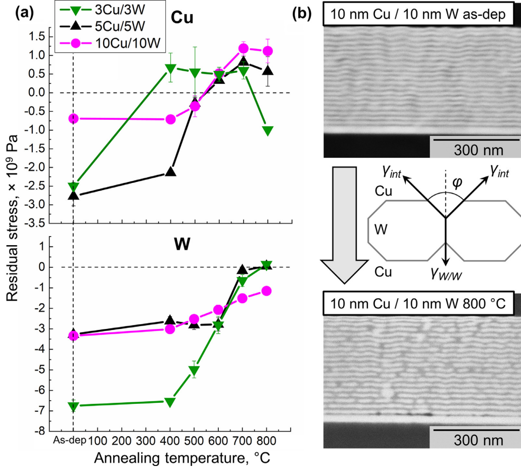
Fig. 1. (a) The evolution of residual stresses in NMLs upon thermal treatment, originally presented in Fig. 9 in Ref. [7] ; (b) schematics of W/W GB grooving and HR-SEM images of 10Cu/10W NMLs in the as-deposited state and after 800°C annealing with pinched-off W nanolayers (the onset of degradation). Error bars are calculated from the linear fit of the strain as a function of \sin^2\psi .
