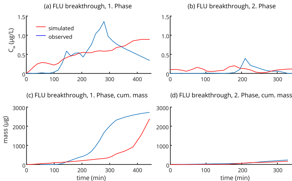
Figure 7. LAST-Model results of FLU breakthrough simulations with FLU concentrations C_w in the tile-drain tube of the field site. (a) and (b) show FLU concentration changes over time and (c) and (d) present cumulated FLU masses in the two irrigation phases, respectively (cf. Sect. 4.1.4 and 4.2.4).
