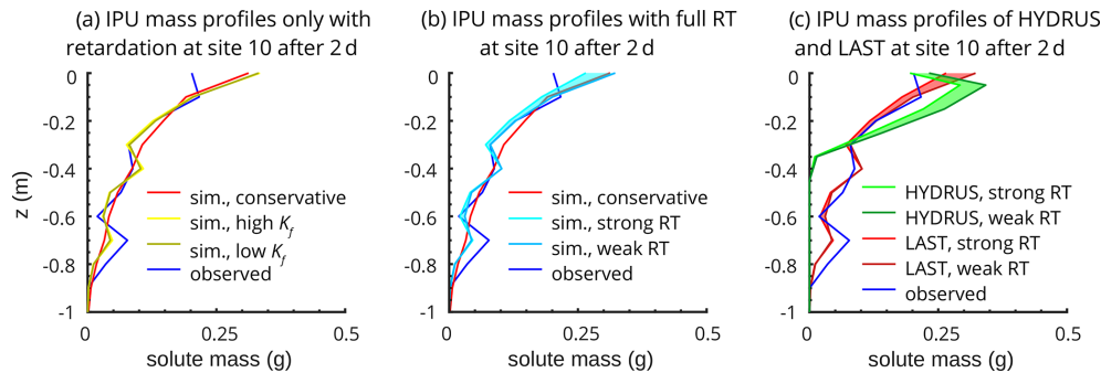
Figure 5. LAST-Model results of reactive IPU transport simulations at the preferential-flow-dominated site (site 10) after 2 d. (a) The simulation is performed only with active retardation and with low and high values for K_f . (b) The simulation is performed with activated retardation and degradation. The shaded area between the profiles with weak and strong reactive transport (cf. Table 2) shows the uncertainty area of the empirical K_f and DT50 values. (c) Comparison with HYDRUS 1-D simulation results.
