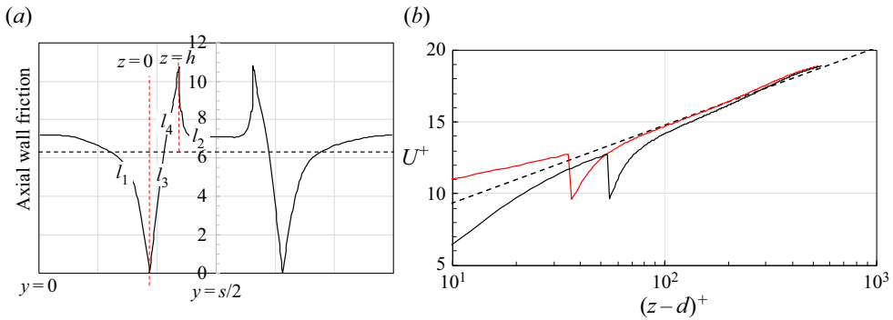
Figure 17. (a) Axial surface stress (in arbitrary units) along one span of the repeating unit within the channel. The sidewall variation at y = (S - W)/2 , between z = 0 and z = h is shown between the two red vertical dashed lines and the sections corresponding to the four integrals I_{1-4} are labelled appropriately. The horizontal dashed line shows the value of the average stress. (b) Axial velocity profile (intrinsically averaged below z = h ). The black and red lines have d/h = 0 and 0.34 , respectively, and the dashed line is the modified log-law (as in figure 2a).
