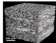
CT-Scan of glass fiber orientation in a FRP
