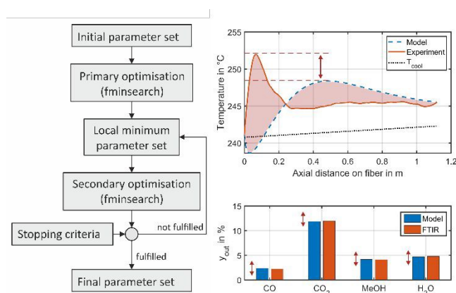
Figure 3: Illustration of parameter fitting applied in this study (left) and an exemplary working point a benchmark conditions at 50 bar showing the temperature profile (right, top) and gas phase molar fractions (right bottom) obtained from the experiment (solid, red) and the miniplant reactor simulation (dotted, blue) using the original kinetic model by Nestler 27 ; Red arrows and area indicate errors minimized by the parameter fitting; The measured temperature profile is smoothed by the Savitzky-Golay filter 67 .
