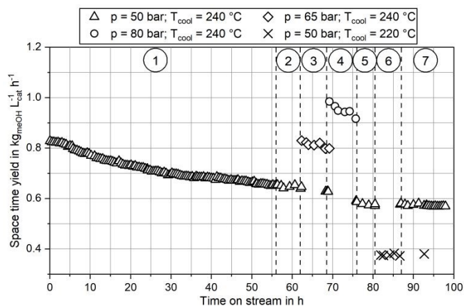
Figure 4: Trend of the space time yield over time-on-stream at benchmark conditions COR = 0.9; SN = 4.0; GHSV = 12,000 h -1 at 50 bar, 65 bar and 80 bar at T cool = 240 °C and T cool = 220 °C. Sectors marked: 1.) ramp up, benchmark at 50 bar, 240 °C; 2.) experimental plan at 50 bar and 240 °C; 3.) experimental plan at 65 bar and 240 °C; 4.) experimental plan at 80 bar and 240 °C; 5.) variation of SN at COR = 0.98, 240 °C and 50 bar to 80 bar; 6.) experimental plan at 50 bar, 220 °C; 7.) benchmark at 50 bar, 240 °C.
