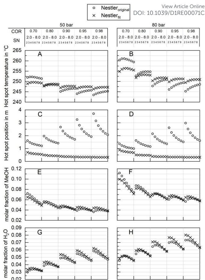
Figure 9: Sensitivity study discussing the behaviour of Nestler original kinetic model (o) and the herein proposed model Nestler fit (x) by means of hot spot temperature (A, B), hot spot position (C, D), product molar fraction of methanol (E, F) and product molar fraction of water (G, H) at a synthesis pressure of 50 bar (A, C, E, G) and 80 bar (B, D, F, H) in the range 0.7 \leq \text{COR} \leq 0.98 , 2.0 \leq \text{SN} \leq 8.0 at \text{GHSV} = 6,000 \text{ h}^{-1} .
