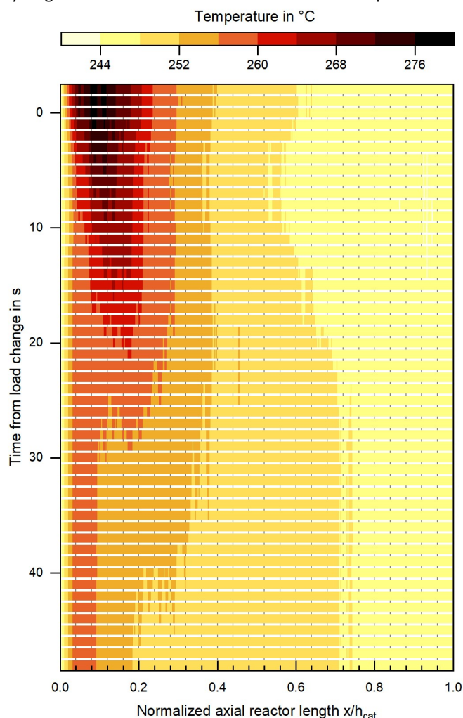
Figure 11: Change in temperature profile during a dynamic load change at a pressure level of 80 bar and T cool = 240 °C from COR = 0.8; SN = 2.0; GHSV = 6,000 h -1 towards COR = 0.9; SN = 4.0; GHSV = 12,000 h -1 ; The load change was applied to the reactor at t = 0 s.
