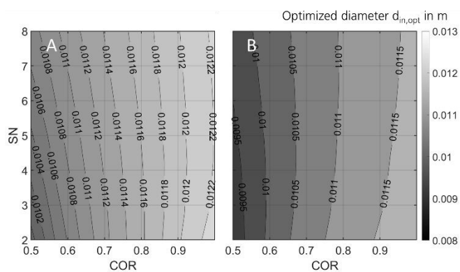
Figure 10: Optimized miniplant reactor diameter over COR and SN at GHSV = 9,000 h -1 and T cool = 240 °C for maximised comparability towards industrial scale at 50 bar (A) and 80 bar (B).
