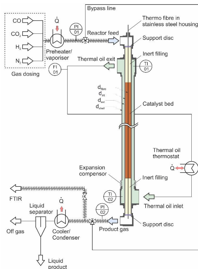
Figure 2: Simplified flow sheet of the experimental setup.
