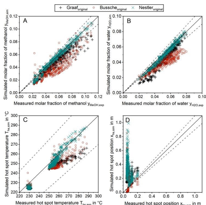
Figure 7: Parity plots for the outlet molar fractions of methanol (A), outlet molar fraction of water (B), hot spot temperature (C) and axial hot spot position (D) including error lines for 0% (solid line) and for 10% (dashed line); Experiments were carried out at the miniplant setup; Simulation was carried out using the kinetic models by Graaf (+), Bussche (o) and Nestler (x) as published.
