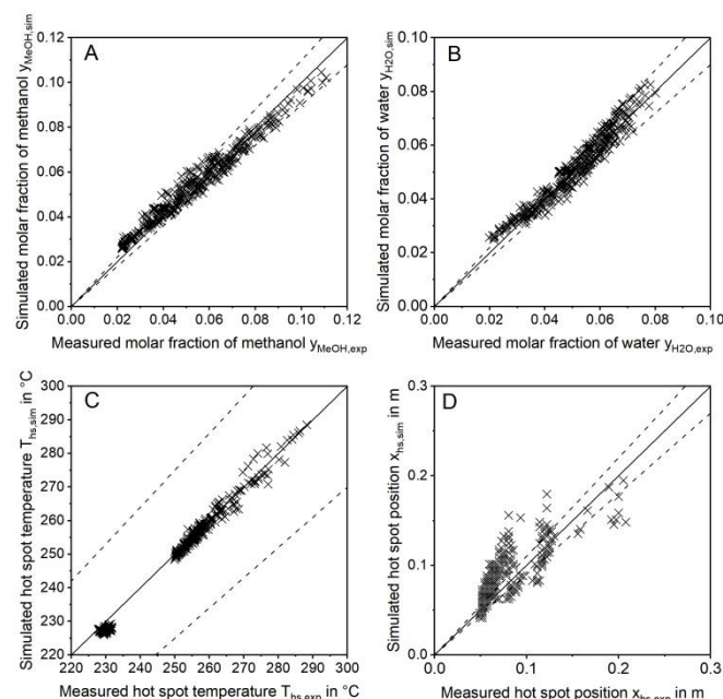
Figure 8: Parity plots of the refitted kinetic model Nestler fit for outlet molar fractions of methanol (A), outlet molar fraction of water (B), hot spot temperature (C) and axial hot spot position (D) including error lines for 0% (solid line) and for 10% (dashed line); Experiments were carried out at the miniplant setup.
