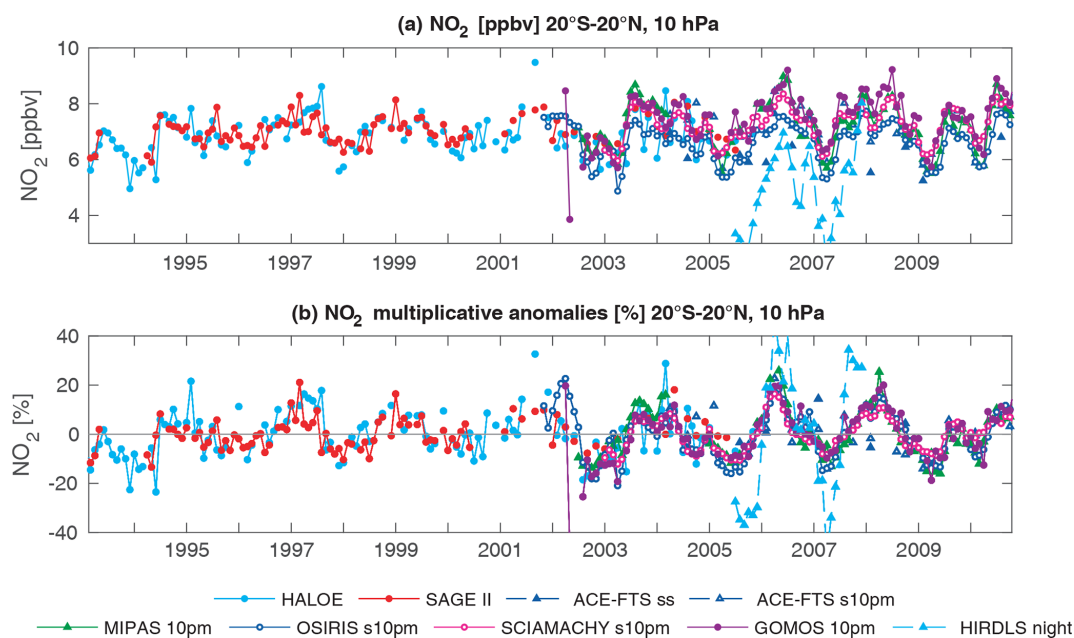
Figure 13. Time series of tropical NO 2 mean values (a) and deseasonalized anomalies (b) between 20° S–20° N at 10 hPa for 1993–2010. Datasets correspond to local sunset or to 22:00 LST as described in the text. The s10pm denotes zonal monthly mean fields scaled to 22:00 LT, the ss zonal monthly mean fields from sunset measurements.
