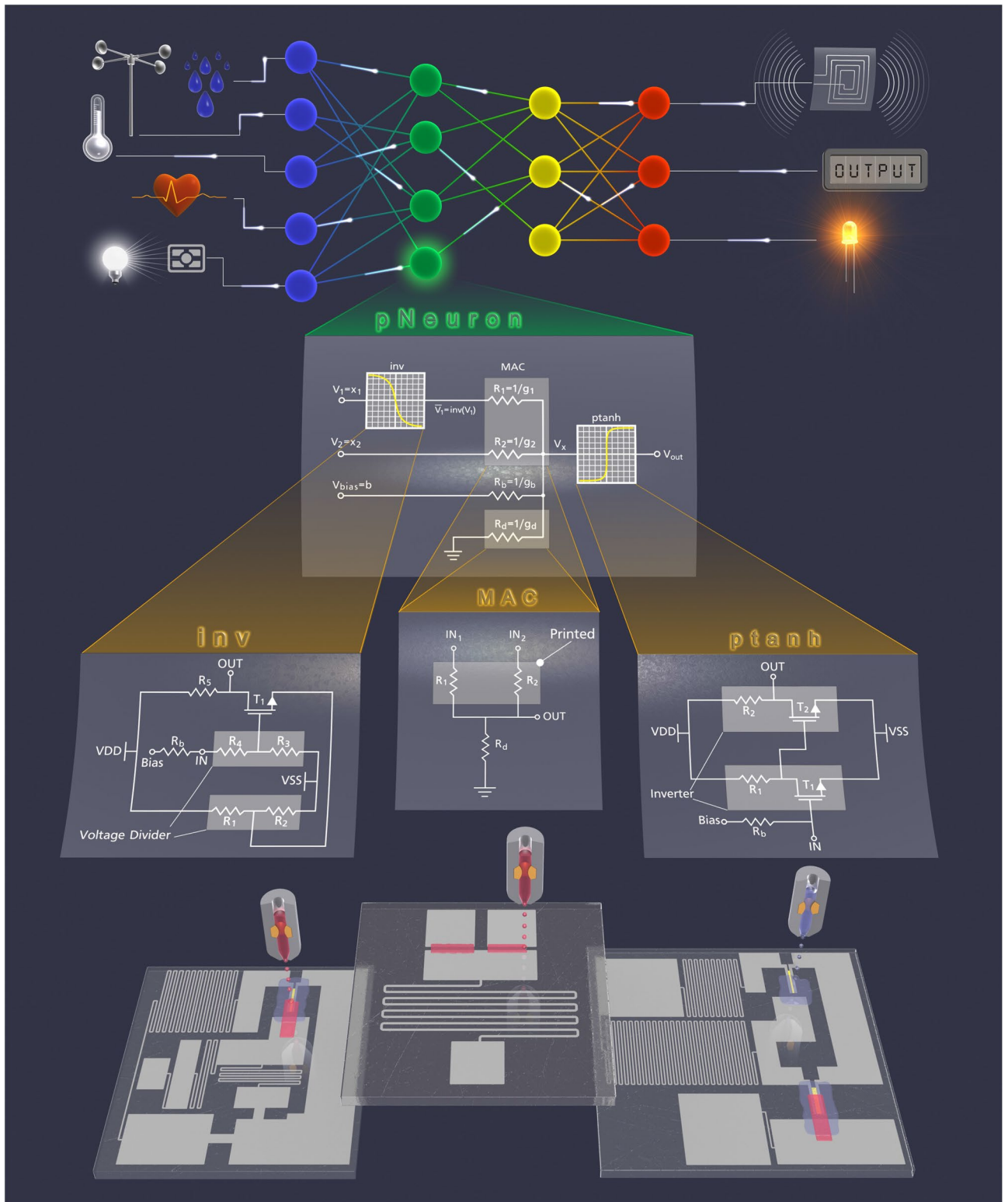
Figure 1. Top: Printed Neural Network with sensor inputs and actuators, Middle: circuit schematics of the inkjet-printed neuron (pNeuron) and the hardware prototypes of its three fundamental building blocks: negative weights circuit (inv), multiply accumulate operation (MAC) and non-linear tanh-like activation function (ptanh) Bottom: physical layout of the hardware prototypes.
