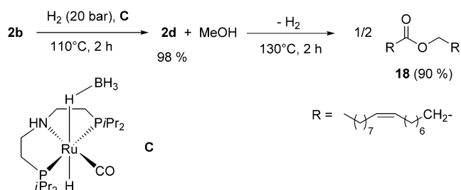
Scheme 2. Synthesis of oleyl oleate 18 by consecutive hydrogenation–dehydrogenation reaction of 2b . [21]
