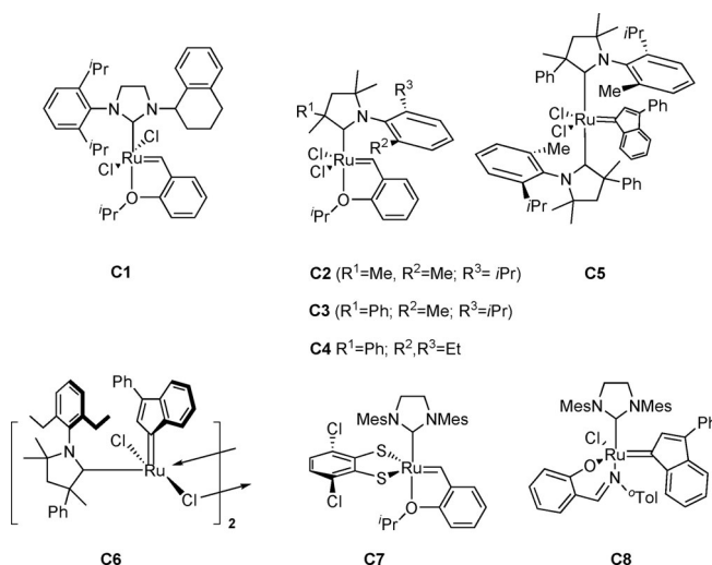
Scheme 18. Ruthenium-based metathesis precatalysts used for the transformation of fatty acid derivatives.
