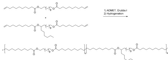
Scheme 23. Branched polyesters, derived from castor and vernonia oil, mimicking the structure and properties of olefin-based elastomers. [147]
