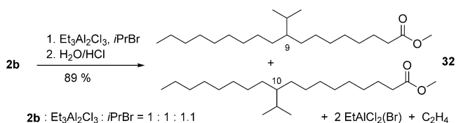
Scheme 11. Et 3 Al 2 Cl 3 -mediated hydroisopropylation of 2b . [60]
