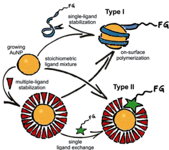
Fig. 1. Illustration of the two strategies geared towards monofunctionalized AuNPs considered in this review. FG = functional group.
