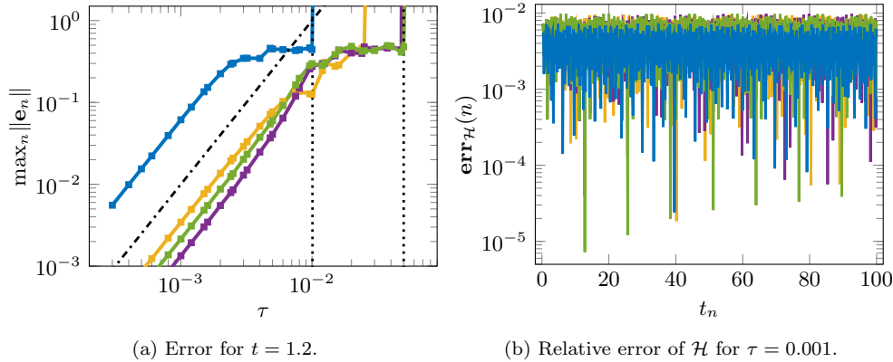
Fig. 6.2: Error (left) and relative error of Hamiltonian (right) for the numerical solution of the FPUT \beta -problem. For \Psi = \Psi_p we use polynomial degrees p = 3 , p = 5 , p = 6 and as stabilization parameter \eta = 0.5 . The blue lines represents the LF scheme. In the left plot the dash-dotted line indicates order two, the dotted lines correspond to the "maximal stable" step size for the LF scheme applied to the stiff system (1.1) and to the nonstiff problem (1.1) with \mathbf{S} = \mathbf{K} = 0 . In the right plot the relative error of the Hamiltonian is plotted only at every 200th time step for the sake of clarity.
