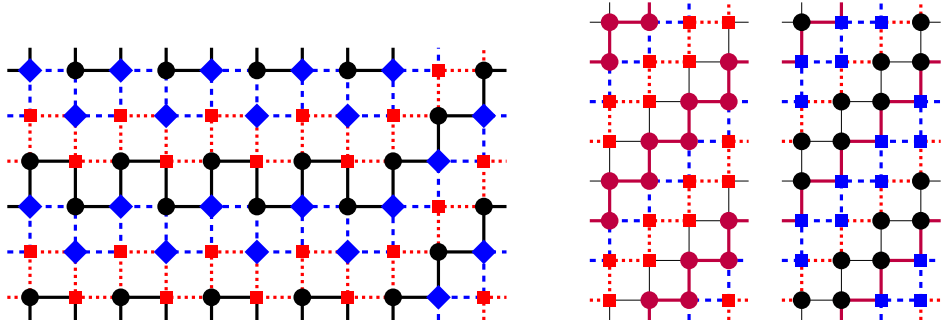
Fig. 3. Left: A 3-DR-splittable cycle decomposition of C_6 \square C_{11} produced by the 3-wiggle decomposition. There is one splitting set, \mathcal{F}_1 , containing all three cycles (dotted red, dashed blue, and black). The red square vertices, blue diamond vertices, and black circular vertices are the representing sets for the cycles with the corresponding color. Right: A 2-DR-splittable cycle decomposition of C_8 \square C_4 produced by the 4-wiggle decomposition. There are two splitting sets: \mathcal{F}_1 contains the dotted red and thick purple cycles, and the representing sets for these cycles are the square red and circular purple vertices illustrated on the left, while \mathcal{F}_2 contains the dashed blue and thin black cycles, and the representing sets for these cycles are the square blue and circular black vertices illustrated on the right. (For interpretation of the references to color in this figure legend, the reader is referred to the web version of this article.)
