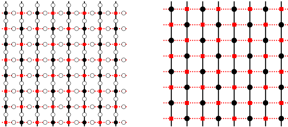
Fig. 8. An illustration of the assignment of the degree four vertices in the subdivided tori to representing sets in Proposition 11. Left: The red square vertices are in the representing set for the red dotted horizontal cycles, and the black circular vertices are in the representing sets for the vertical black cycles. Right: The corresponding cycles and vertices in the underlying torus. (For interpretation of the references to color in this figure legend, the reader is referred to the web version of this article.)
