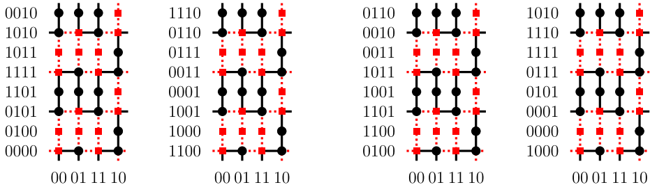
Fig. 7. A 4-splittable decomposition of Q_6 into eight cycles of the same length. \mathcal{F}_1 contains the four cycles on the left two subdivided tori, where the red square vertices and the black circular vertices are the representing sets for the red dotted and black cycles, respectively. \mathcal{F}_2 contains the four cycles on the right two subdivided tori, with the same color scheme for cycles and representing sets. (For interpretation of the references to color in this figure legend, the reader is referred to the web version of this article.)
