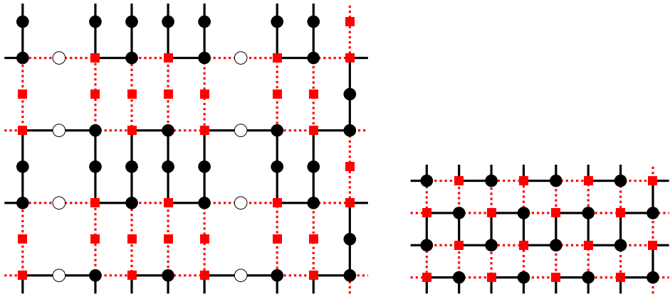
Fig. 5. Left: A 2-wiggle decomposition of a subdivided torus (C, S) \boxplus (C', S') into two cycles C_1 and C_2 (black and dotted red). Note that since (C, S) is distance regular (though (C', S') is not) the cycles have the same length. In the notation of Proposition 6, the black circular vertices are in S_1 and the red square vertices are in S_2 . Note that the vertices in S_1 are on the cycle C_1 , and S_1 and S_2 partition the vertices of C \square S' . Right: The 2-wiggle decomposition on the underlying torus, where every other vertex on a given cycle is in its representing set.
