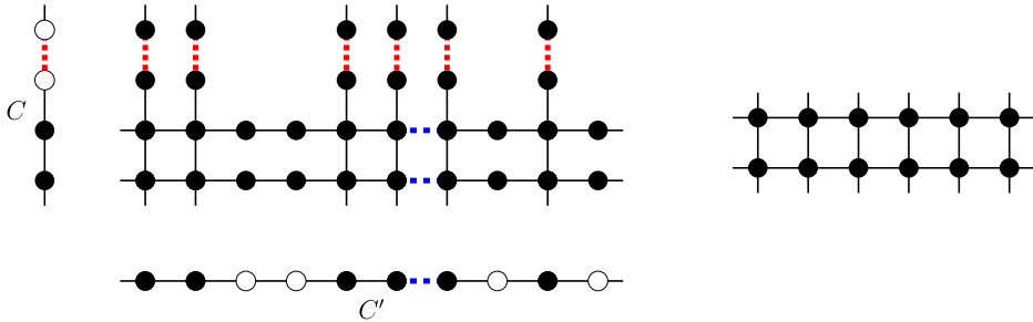
Fig. 1. Left: Two cycles C = (0, 1, 2, 3, 0) and C' = (0, 1, 2, 3, 4, 5, 6, 7, 8, 9, 0) , and the anchored product (C, S) \boxplus (C', S') , where S = \{0, 1\} and S' = \{0, 1, 4, 5, 6, 8\} . A given row and column of the anchored product are highlighted in dotted red and dashed blue, respectively, along with the corresponding edge from the original cycle. Right: The underlying torus of (C, S) \boxplus (C', S') .
