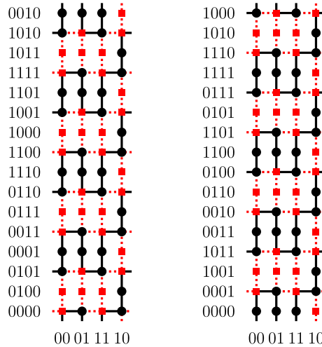
Fig. 6. A 2-splittable decomposition of Q_6 into four cycles of the same length. \mathcal{F}_1 contains the two cycles on the left (black and dotted red), where the red square vertices and the black circular vertices are the representing sets for the cycle with the same color. \mathcal{F}_2 contains the two cycles on the right, with the same color scheme for cycles and representing sets. (For interpretation of the references to color in this figure legend, the reader is referred to the web version of this article.)
