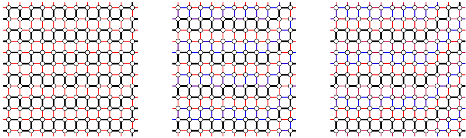
Fig. 2. Left: The 2-wiggle decomposition of C_{12} \square C_{12} into two cycles (red and thick black). Middle: The 3-wiggle decomposition of C_{12} \square C_{11} into three cycles (red, blue, and thick black). Right: The 4-wiggle decomposition of C_{12} \square C_{12} into four cycles (purple, blue, red, and thick black). (For interpretation of the references to color in this figure legend, the reader is referred to the web version of this article.)
