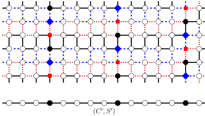
Fig. 4. An example for Proposition 5: The 3-wiggle is applied to C \square C' = C_6 \square C_{15} , to produce a decomposition into three cycles C_1, C_2 , and C_3 (dotted red, dashed blue, and black). In this example S' = \{3, 8, 13\} , and the vertices in C \times S' are partitioned into sets S_1, S_2 , and S_3 (red squares, blue diamonds, black circles). Note that each path in C' between consecutive elements of S' has length 5, and each path in C_1 between consecutive vertices in S_1 has length 10.
