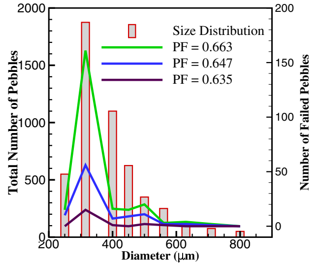
Fig. 7 Size distribution of the pebbles and number of failure pebbles at the end of 1.5% strain ( a = 2 ). The bar shows the total number, and the lines indicate number of failed pebbles
