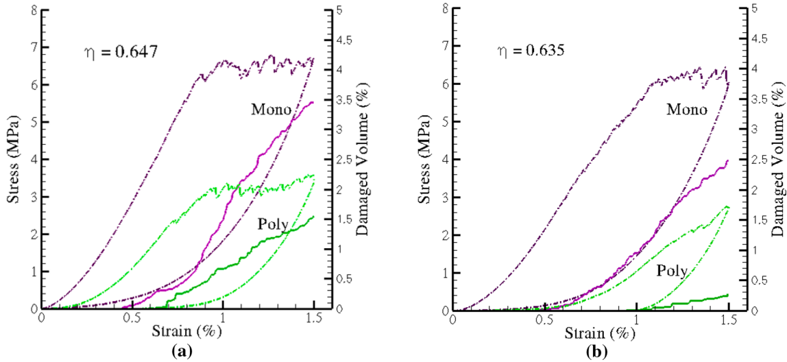
Fig. 6 Macroscopic stress response and damaged volume (%) as a function of strain for various mono and polydispersed systems for a = 2
