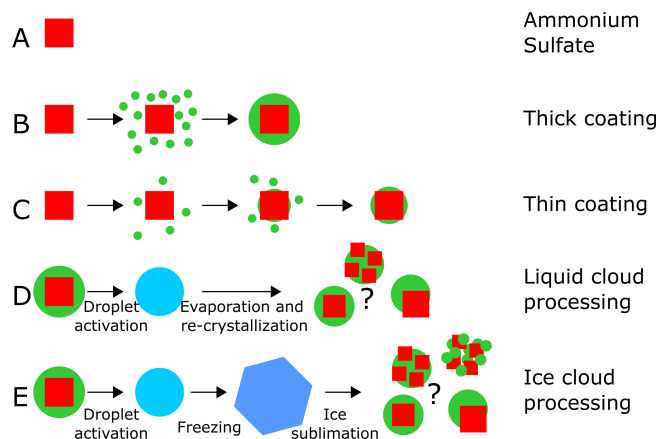
Figure 1. Summary of the experiments performed. Experiment A: crystalline ammonium sulfate (AS). Experiment B: AS crystals thickly coated with secondary organic matter (SOM) from the ozonolysis of \alpha -pinene (AP) at +20^\circ\text{C} in the aerosol preparation and characterization (APC) chamber (thick coating). Experiment C: AS crystals stepwise coated with small amounts of SOM from the ozonolysis of AP at upper tropospheric temperature in the AIDA chamber (thin coating). Experiment D: in situ crystallization of the AS component from a homogeneously mixed, aqueous droplet that was generated by the droplet activation of crystalline AS aerosol thickly coated with SOM (prepared as in experiment B). Experiment E: aerosol prepared in the same way as in B but then subjected to an atmospheric freeze-drying process, involving droplet activation, freezing, and ice sublimation. A detailed description of the experiments is provided in the main text.
