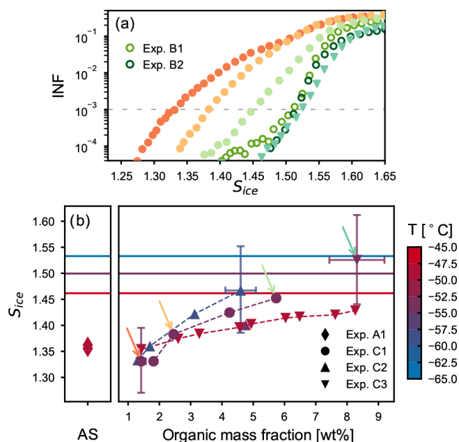
Figure 6. Ice nucleation results for the thin coating experiments (type C). (a) Ice-nucleating fraction as function of S_{ice} for humidity scans performed with INKA at \sim -54^\circ\text{C} during experiments C1 (solid circles), C3 (down-pointing triangles), and B (empty circles). (b) Ice onsets saturation ratio (defined for an INF of 0.1%) for all INKA measurements during experiments C1, C2, and C3. Colors indicate the temperature at which the ice nucleation measurements have been performed in INKA. The horizontal lines indicate the threshold for homogeneous freezing of solution droplets at three different temperatures ( \Delta a_w = 0.3 , Koop et al., 2000). In all experiments, a gradual increase in the ice onset saturation ratios with increasing organic mass fraction was measured (dashed lines to guide the eyes). The colored arrows indicate the measurements reported in panel (a).
