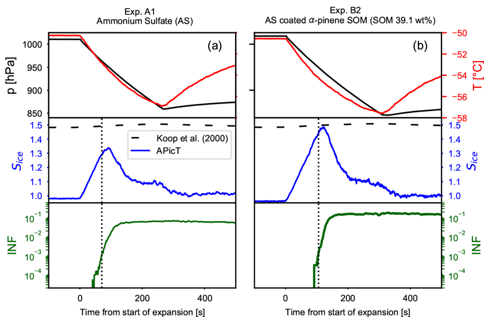
Figure 4. Time series of the AIDA expansion cooling experiments for (a) pure crystalline ammonium sulfate (experiment A1) and (b) ammonium sulfate crystals coated with SOM from the ozonolysis of \alpha -pinene (experiment B2). The upper panels show pressure (black lines, left axis) and temperature (red lines, right axis). The middle panels show the increase in the saturation ratio with respect to ice (blue line). The homogeneous freezing threshold computed for a \Delta a_w of 0.3 of the ice-melting curve (Koop et al., 2000) is indicated with the horizontal dashed lines. The lower panels show the fraction of aerosol particles that induced ice formation (ice-nucleating fraction, INF). The vertical dotted lines indicate when 0.1 % of the aerosol particles acted as INPs.
