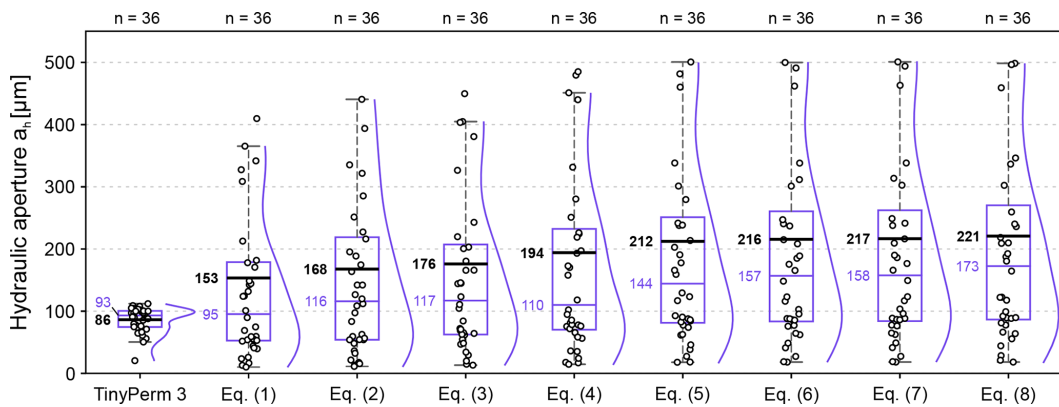
Figure 5. Comparison of hydraulic fracture apertures measured by the air permeameter (TinyPerm 3) and estimated based on mean mechanical fracture apertures and standard deviations from microscopic fracture trace analysis. For each dataset, the arithmetic mean (bold black line), the median (thin purple line) and the probability density function (obtained by kernel density estimation) are shown. Values above 550 \mu\text{m} are excluded from the graph.
