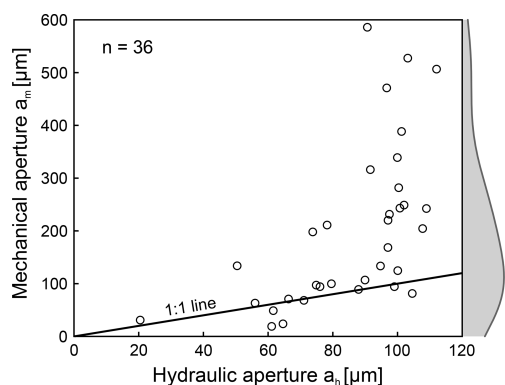
Figure 4. Comparison of measured mechanical and hydraulic fracture apertures in the EZ-B niche with probability density function for a_m . Two outliers with mechanical apertures of 789 and 833 \mu\text{m} are not shown for better visibility.
