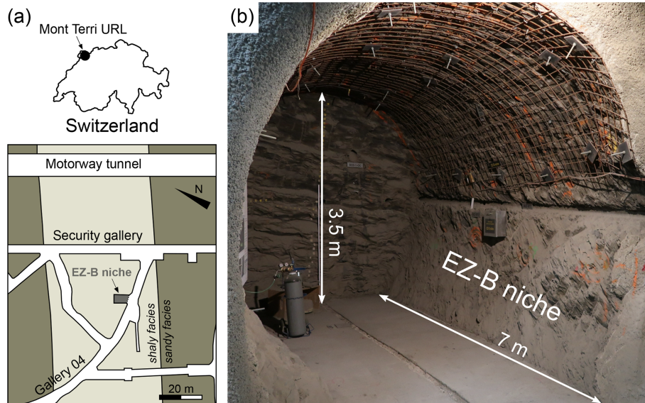
Figure 1. (a) Location of the Mont Terri underground rock laboratory (URL) alongside the security gallery of the Mont Terri motorway tunnel and the EZ-B niche situated in the shaly facies of the Opalinus Clay. (b) Photo and dimensions of the EZ-B niche where data acquisition was conducted. In the entrance area, shotcrete partly covers the rock surface on the left and right side wall.
