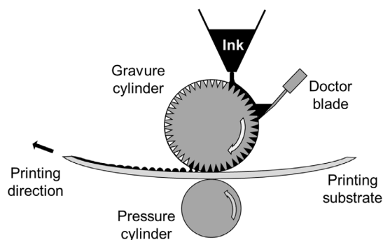
Figure 1. Schematic illustration of the gravure printing process.
