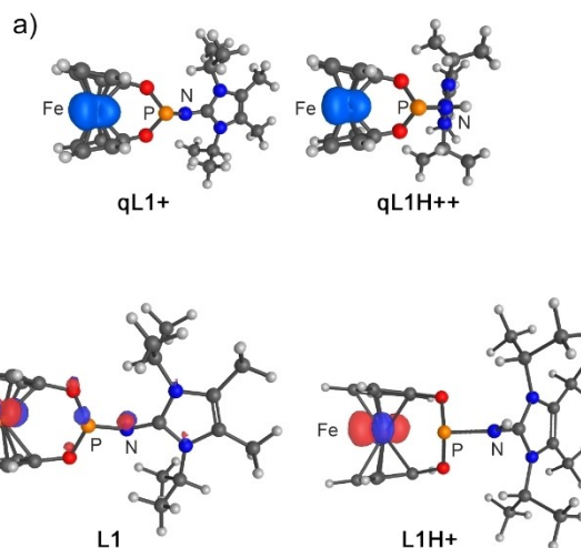
Figure 7. a) Calculated spin density of the oxidized proligands qL1 + and qL1H ++ , iso value: 0.002. b) HOMOs of L1 and L1H + , iso-value 0.075.
