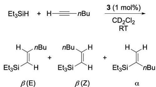
Scheme 5. Catalytic hydrosilylation of hex-1-yne with triethyl silane using [\text{L1Rh}(\text{cod})\text{Cl}] ( 3 ) as precatalyst.
