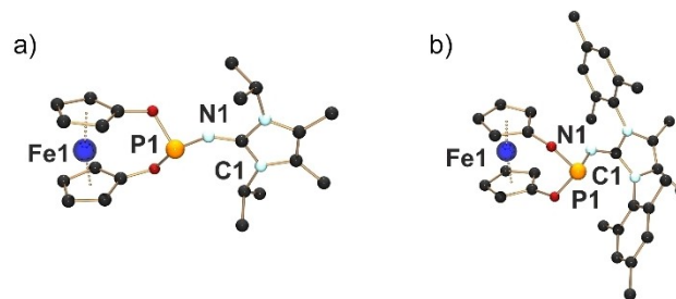
Figure 2. Molecular structures of a) L1 [a] and b) L2 . H atoms are omitted for clarity. Selected distances [pm]: L1 : Fe1...P1 343.7, P1-N1 159.7; L2 : Fe1...P1 358.7, P1-N1 163.9. [a] L1 crystallizes with two molecules in the asymmetric unit. Distances are given as the average of both.
