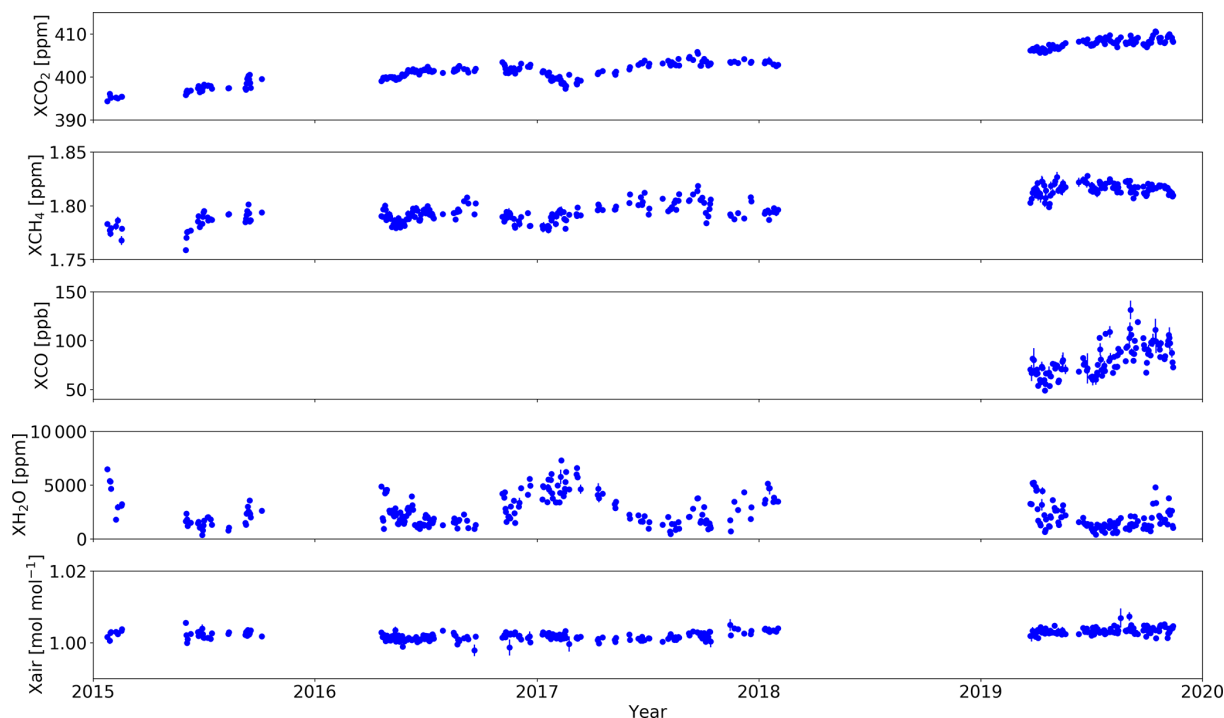
Figure 5. Column-averaged dry-air mole fraction time series for X_{\text{CO}_2} , X_{\text{CH}_4} , X_{\text{CO}} , X_{\text{H}_2\text{O}} and X_{\text{air}} measured at the COCCON site in Gobabeb, Namibia, from January 2015 until November 2019. Daily mean values are shown for better visibility. Error bars denote the 1\sigma standard deviation of the daily mean values. In 2018, the instrument was upgraded with a second channel. Therefore, X_{\text{CO}} observations only started in 2019.
