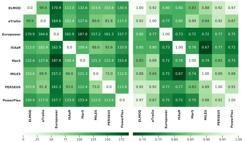
Figure 4.4: RMSE of PV installed capacities differences (MW) across all NUTS 3 regions (left) and mean Pearson correlation of PV profiles across intersecting NUTS 3 regions (right).
