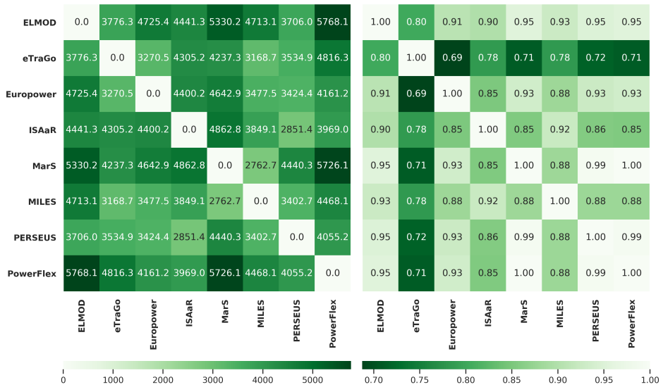
Figure B.4: RMSE of annual load (GWh) differences across all NUTS 2 regions (left) and mean Pearson correlation of load profiles across intersecting NUTS 2 regions (right).
