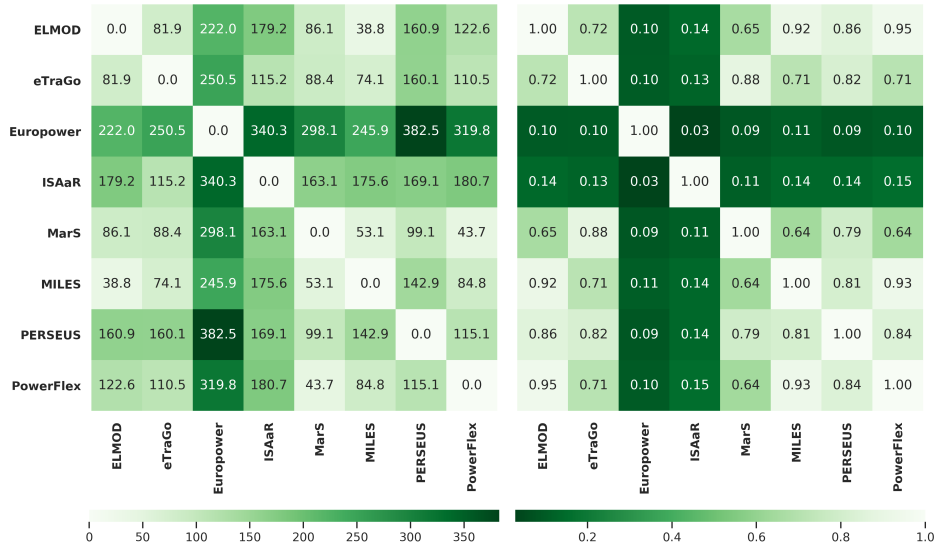
Figure B.3: RMSE of wind offshore installed capacities differences (MW) across all NUTS 2 regions (left) and mean Pearson correlation of wind offshore profiles across intersecting NUTS 2 regions (right).
