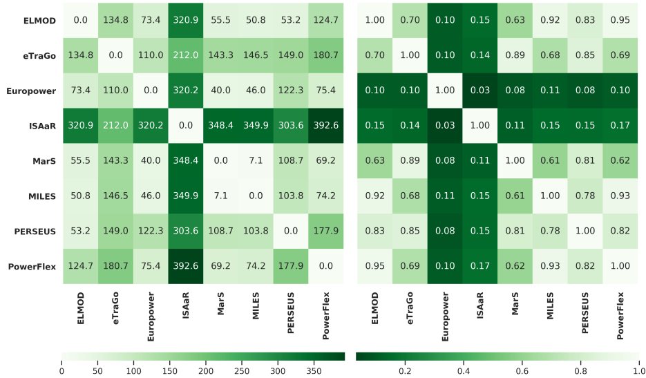
Figure 4.7: RMSE of wind offshore installed capacities differences (MW) of the North sea and the Baltic sea (left) and mean Pearson correlation of the North sea and the Baltic sea wind offshore profiles (right).
