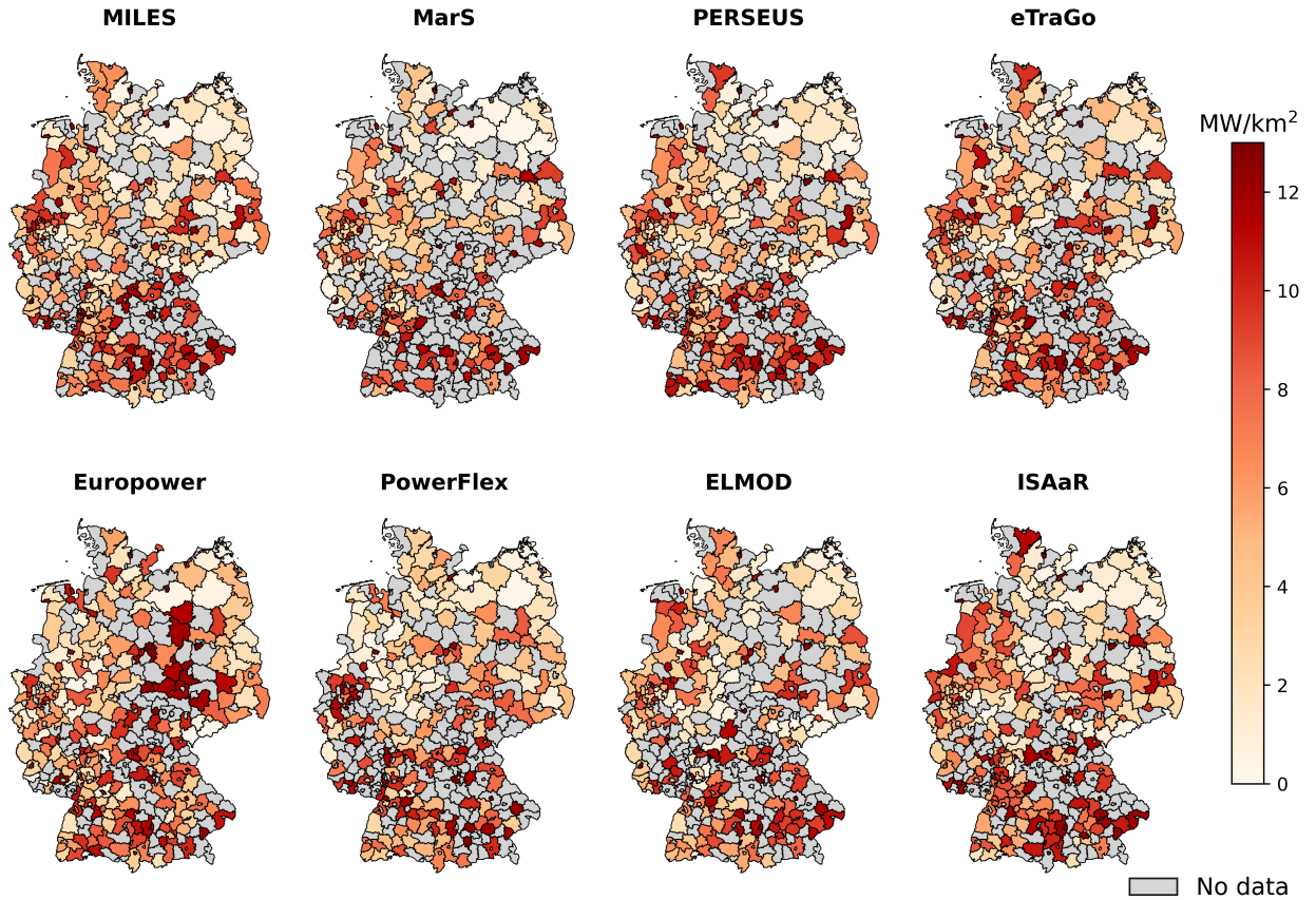
Figure A.1: PV installed capacity at ehv-nodes aggregated per NUTS 3 regions density plot in \text{MW}/\text{km}^2 .
