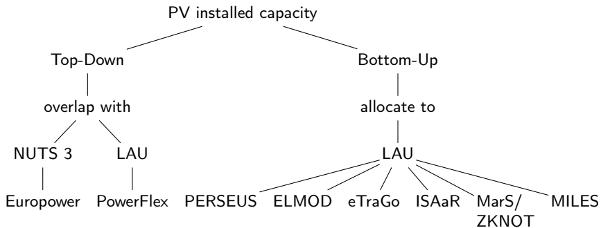
Figure 4.1: Dendrogram of regionalization of PV installed capacity workflows
