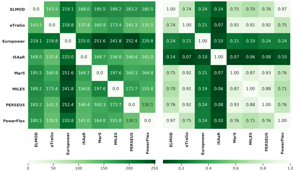
Figure 4.5: RMSE of wind onshore installed capacities differences (MW) across all NUTS 3 regions (left) and mean Pearson correlation of wind onshore profiles across intersecting NUTS 3 regions (right).
