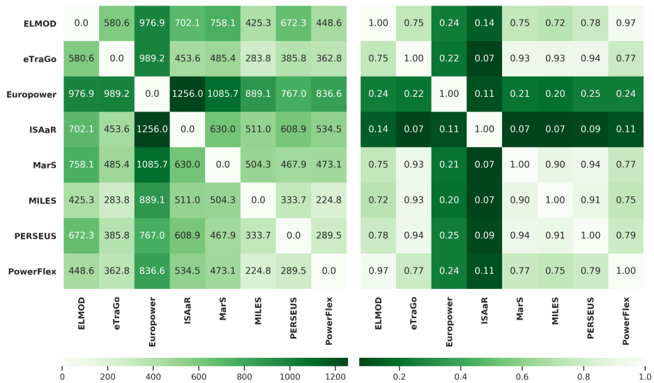
Figure B.2: RMSE of wind onshore installed capacities differences (MW) across all NUTS 2 regions (left) and mean Pearson correlation of wind onshore profiles across intersecting NUTS 2 regions (right).
