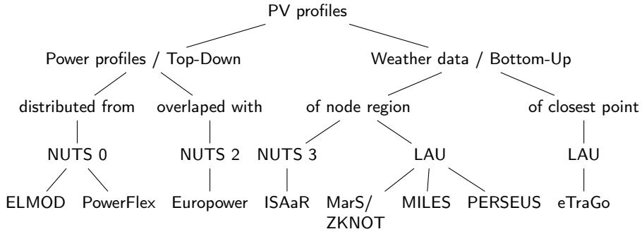
Figure 4.2: Dendrogram of regionalization of PV profiles workflows.
