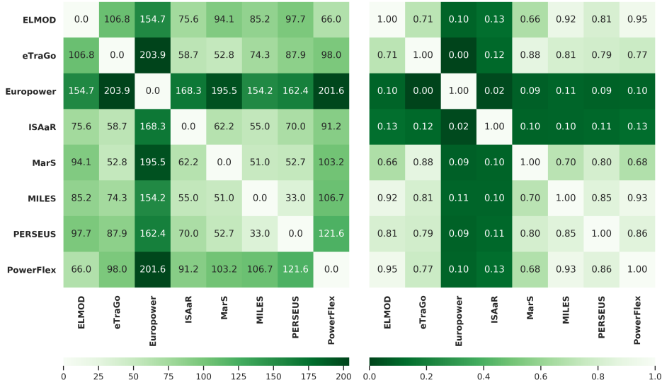
Figure 4.6: RMSE of wind offshore installed capacities differences (MW) across all NUTS 3 regions (left) and mean Pearson correlation of wind offshore profiles across intersecting NUTS 3 regions (right).
