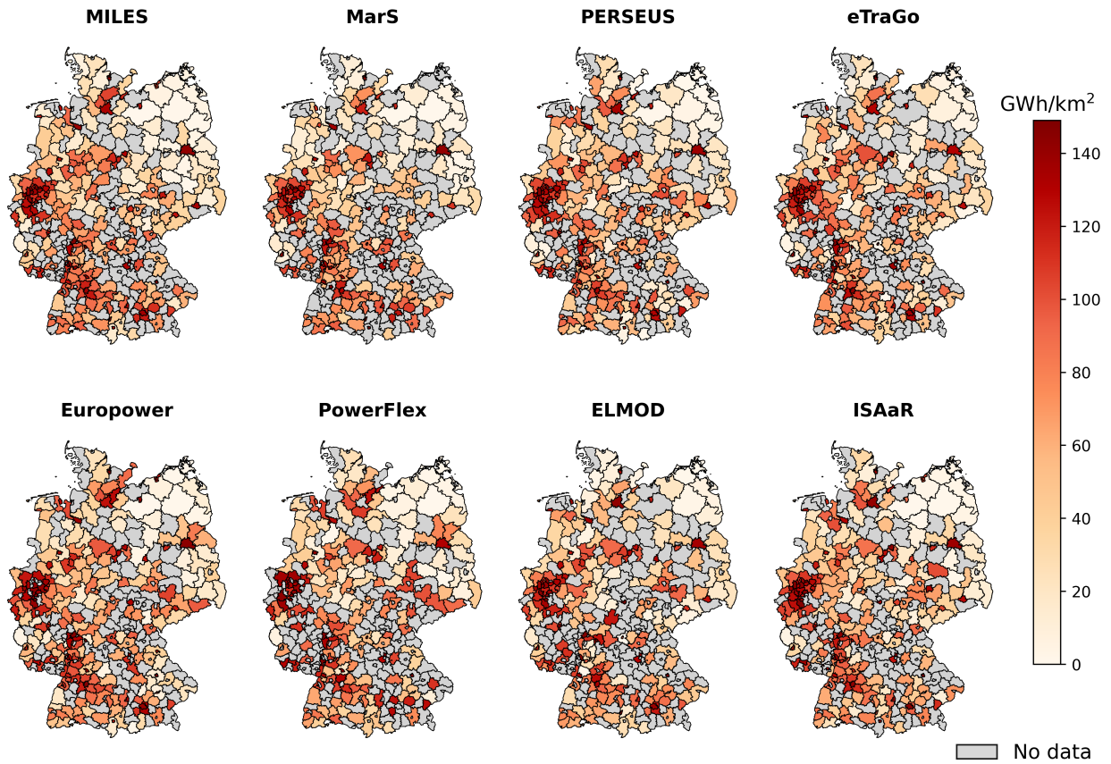
Figure A.4: Annual demand installed capacity at ehv-nodes aggregated per NUTS 3 regions density plot in GWh/km 2 .
