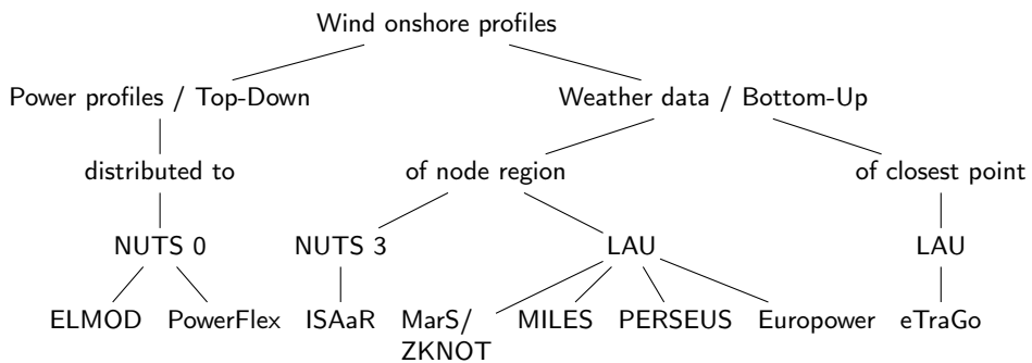
Figure 4.3: Dendrogram of the regionalization of wind onshore profiles workflows
