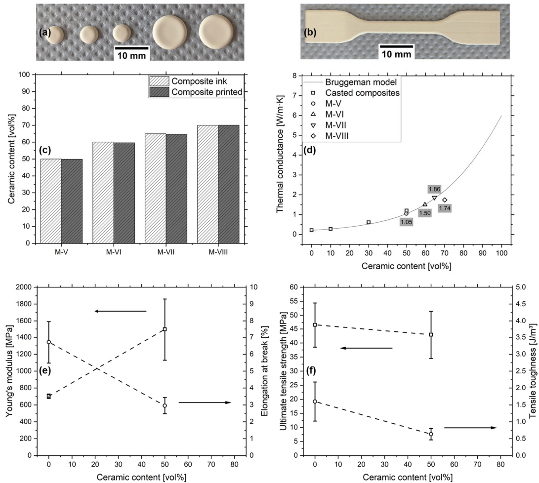
Figure 5. (a) Specimens for the thermal conductance measurement and (b) for the tensile test. (c) Ceramic content of the M-V to M-VIII inks and printed composites. (d) Thermal conductance of the casted composites and of M-V to M-VIII in dependency of the ceramic content complemented by the Bruggeman model. (e) Tensile modulus and elongation at break in dependency of the ceramic content. (f) Ultimate tensile strength and tensile toughness in dependency of the ceramic content.
