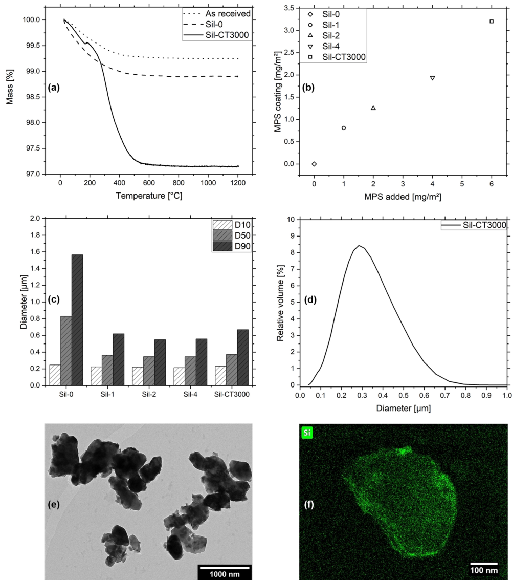
Figure 1. (a) TGA curves of CT3000 as received, Sil-0 and Sil-CT3000. (b) Total amount of MPS in the coating in dependency of the added MPS for Sil-0, Sil-1, Sil-2, Sil-4 and Sil-CT3000. (c) Particle diameters of Sil-0, Sil-1, Sil-2, Sil-4 and Sil-CT3000 expressed in D10, D50 and D90 values. (d) PSD of Sil-CT3000. (e) TEM image of Sil-CT3000. (f) TEM image of a Sil-CT3000 particle with an overlaid EDX signal of silicon.
