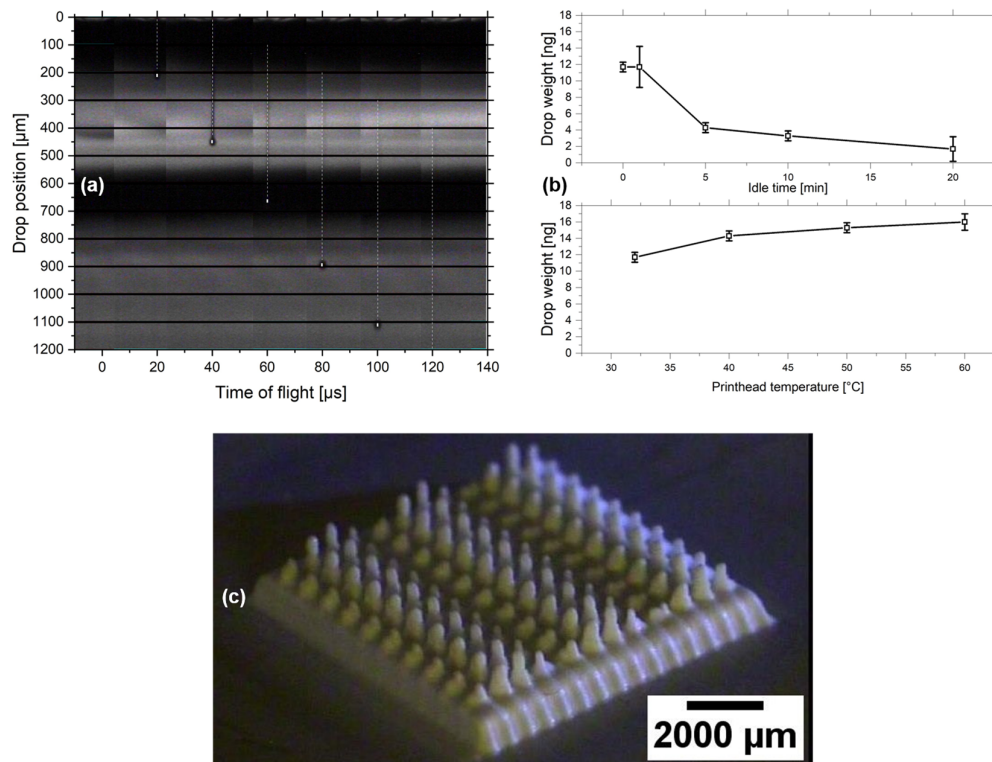
Figure 6. (a) Drop procession during jetting observed over a timeframe of 120 \mu\text{s} . (b) Drop weight of the ink measured as a function of the idle time at 32 ^{\circ}\text{C} and as a function of the printhead temperature. (c) Printed cooling element for the purpose of demonstration.
