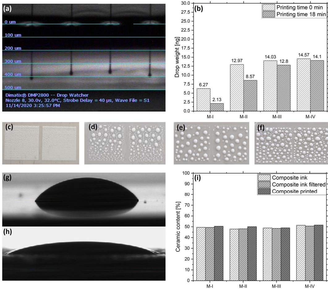
Figure 4. (a) M-IV ink during jetting in the Drop Watcher. (b) Measurement of the average drop weight of M-I to M-IV with 10 nozzles at 32 °C before and after the printing of a test image. (c–f) The four materials deposited onto PDMS with a drop spacing of 20 μm. (g) Drops of the material M-IV on PDMS and (h) on a previously printed and dried film of the same material. (i) Ceramic content of the composite ink before and after filtration, as well as after printing.
