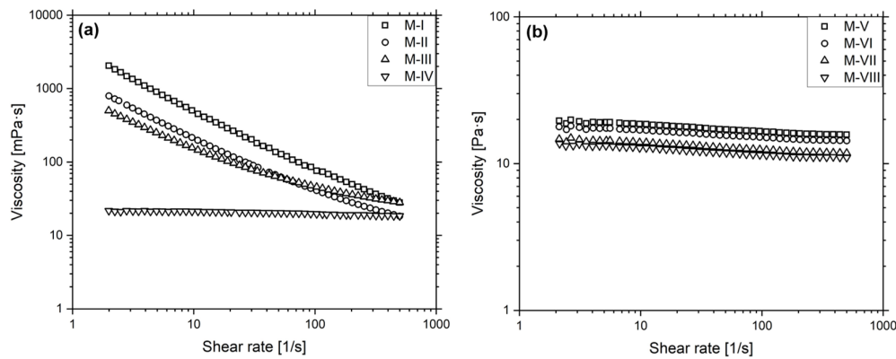
Figure 3. Viscosity of the filtered inks (a) M-I to M-IV and (b) M-V to M-VIII after filtration in dependency of the shear rate at a temperature of 32 °C.
