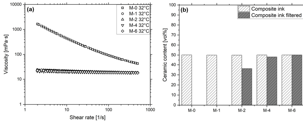
Figure 2. (a) Viscosity in dependency of the shear rate of M-0, M-1, M-2, M-4, M-6 at a temperature of 32 °C. (b) Ceramic content of the materials before and after filtration.
