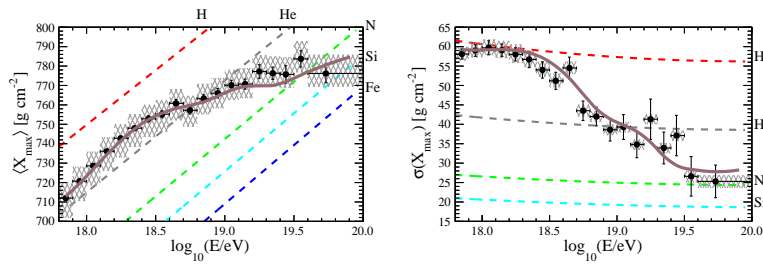
Figure 2: The first two moments of the X_{\text{max}} distributions in each energy bin along with their expected values and the predictions for pure compositions of ^1\text{H} (red), ^4\text{He} (grey), ^{14}\text{N} (green), ^{28}\text{Si} (cyan), ^{56}\text{Fe} (blue).
