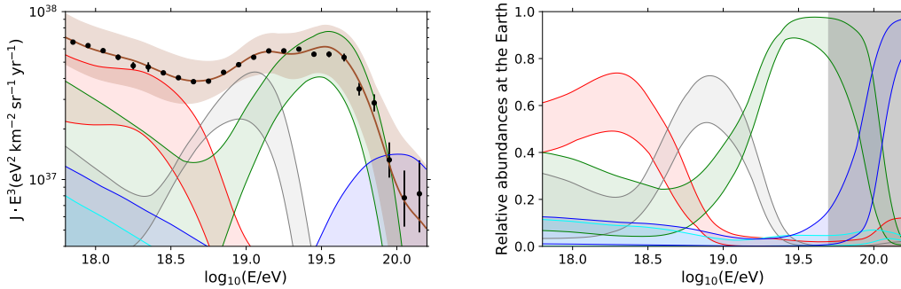
Figure 3: Left: the combined effect of the experimental uncertainties on the energy spectrum. Right: the effect on the relative abundances at the top of atmosphere. The uncertainties are considered by shifting the energies and/or the X_{\max} distributions of 1\sigma_{\text{sys}} in both directions, as shown in Tab. 3. The bands represent the maximal variations induced by considering all the possible combinations of shifts. The shaded area in the right plot indicates the region where the X_{\max} measurements are grouped in one single energy bin because of the low statistics and thus the mass composition predictions are mainly driven by the energy spectrum fit.
