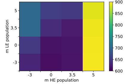
Figure 5: Deviance as a function of the cosmological evolution of the two populations.
