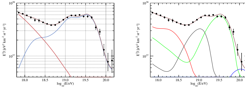
Figure 1: The measured energy spectrum and the estimated best fit results in the scenario with two mixed extragalactic components. Left: the estimated contributions from the two extragalactic components (red: LE component, blue: HE component). Right: the partial fluxes related to different nuclear species at the top of atmosphere, grouped according to their mass number: A = 1 (red), 2 \leq A \leq 4 (grey), 5 \leq A \leq 22 (green), 23 \leq A \leq 38 (cyan), A \geq 39 (blue).
