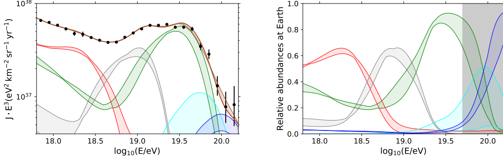
Figure 4: Left: the effect of the uncertainties from models on the energy spectrum. Right: the effect on the relative abundances at the top of atmosphere. The bands represent the maximal variations given by the results in Tab. 4.
