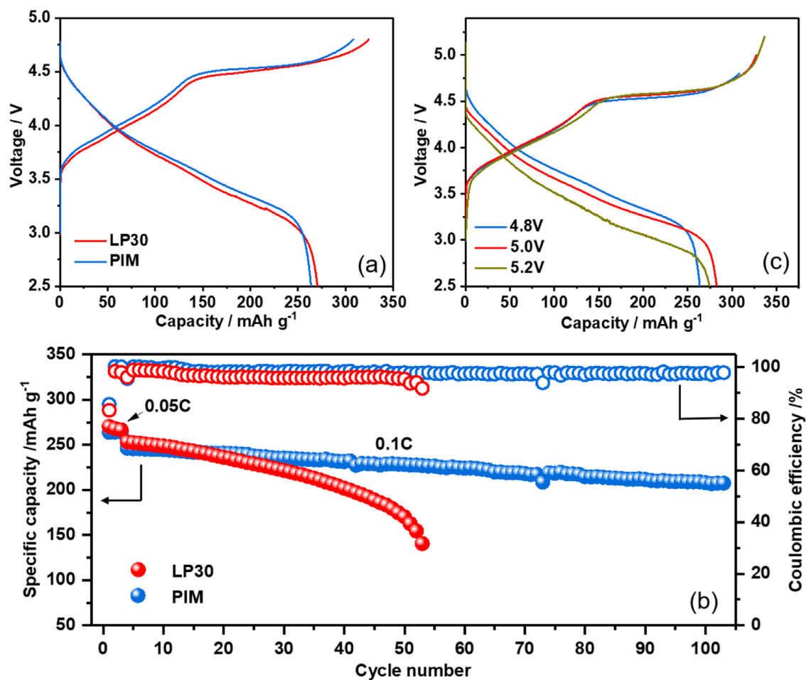
Fig. 6. a) Voltage vs. capacity (1 st cycle) profiles and (b) long-term cycling performance of Li/LRNM cells employing the 0.8\text{P}_{4444}\text{IM}_{14}-0.2\text{LiTFSI} (PIM) and organic carbonate (LP30) electrolytes. c) Voltage vs. capacity profiles obtained for different cut-off voltages for Li/ 0.8\text{P}_{4444}\text{IM}_{14}-0.2\text{LiTFSI} (PIM)/LRNM cells during the first cycle. T = 40^\circ\text{C} .
