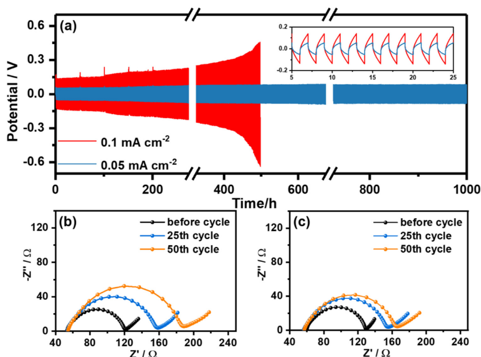
Fig. 5. a) overvoltage/time profiles during galvanostatic cycling ( 0.1 \text{ mA cm}^{-2} and 0.05 \text{ mA cm}^{-2} , with each stripping or plating step lasting for 1 h. Time evolution of the AC responses for Li/ 0.8\text{P}_{4444}\text{IM}_{14}-0.2\text{LiTFSI} (PIM)/Li cells at b) 0.1 \text{ mA cm}^{-2} and c) 0.05 \text{ mA cm}^{-2} . All measurements were performed at T = 40^\circ\text{C} .
