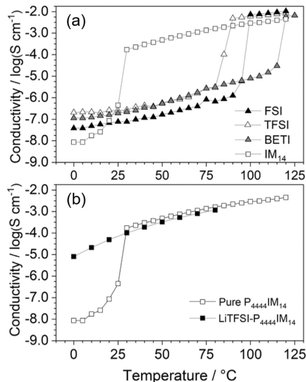
Fig. 3. Ionic conductivity vs. temperature dependence of: a) P 4444 -based ionic liquids with different anions; b) pure P 4444 IM 14 and 0.8P 4444 IM 14 -0.2LiTFSI (PIM) mixture. Scan rate: 1.5 °C h -1 .
