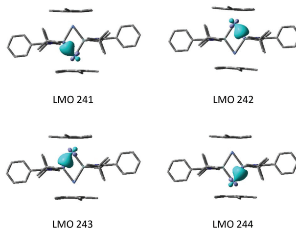
Fig. 3 Isosurface plots (values \pm 0.10 e ) of the localised MOs (LMO 241 to LMO 244) of the \text{Ni}_2\text{Si}_2 molecule showing pronounced Ni–Si bonding.
