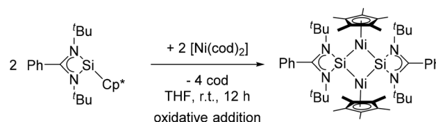
Scheme 1 Synthesis of [\text{PhC}(\text{N}t\text{Bu})_2\text{SiNi}(\text{C}_5\text{Me}_5)_2] .
