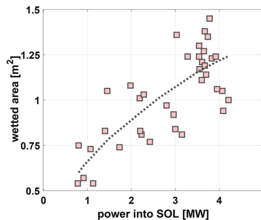
Figure 6. A wetted area as a function of power entering into the scrape-off layer for programs performed in standard configuration [19].
