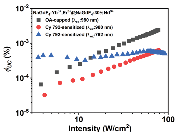
Fig. 6 Intensity dependence of the absolute UC quantum yield for NaGdF 4 :Yb,Er@NaGdF 4 :30%Nd UCNCs: OA-capped UCNCs before ligand dispersed in toluene (black squares); UCNCs after ligand exchange with Cy 792 dye in CD 3 OD under argon and without the purification process excited using a 980 nm (red circles) and a 792 nm (blue triangles) laser.
