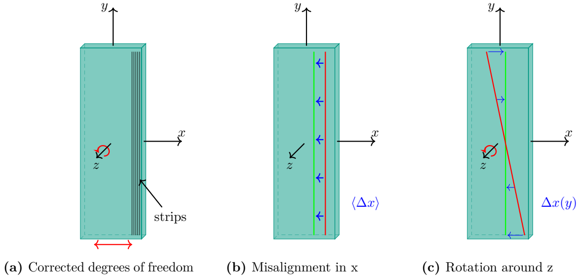
Figure 6.13: Sketch of the DUT post alignment. The alignment step of EUTElescope did not properly corrected the misalignment in x direction and the rotation around the z -axis. The post alignment corrects these degrees of freedom as displayed in (a). The misalignment in x is given by the mean residual \langle \Delta x \rangle of the track position x_{\text{track}} and the recorded cluster position x_{\text{cl}} as visualized in (b). The rotation around the z -axis is the slope of the x residual over the y track position \Delta x(y) as illustrated in (c).
