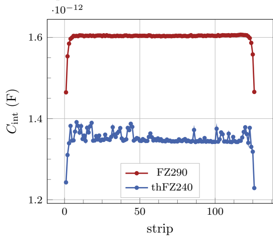
(e) Inter-strip coupling capacitance C_{\text{int}}
