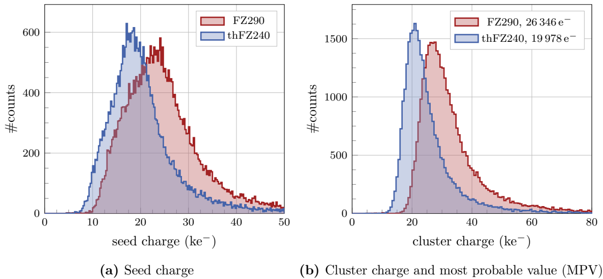
Figure A.9: Comparison of the seed charge (a) and cluster charge (b) for energy depositions of electrons emitted by a ^{90}\text{Sr} source. The measurements were performed in the ALiBaVa setup for thFZ240 and FZ290 sensors at 20 °C and 400 V bias voltage. Since the FZ290 sensors are thicker the electrons create more charge carriers.
