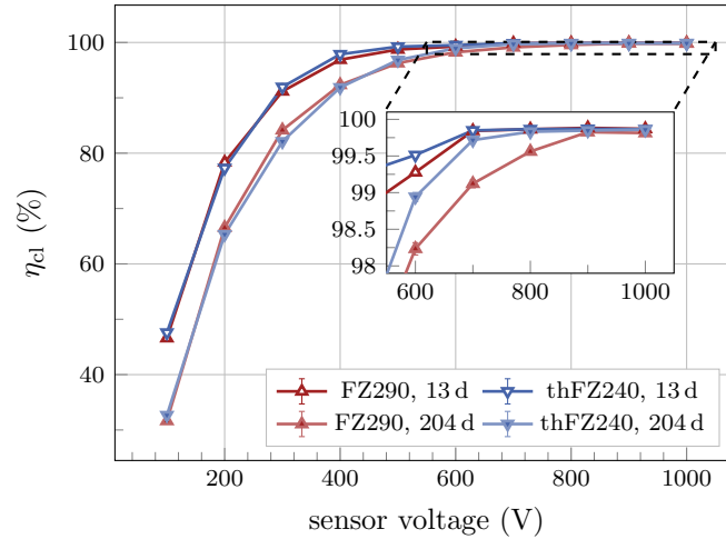
Figure 10.4: Cluster efficiency over the sensor bias voltage for MiMo3 ( 5 \times 10^{14} \text{ n}_{\text{eq}}/\text{cm}^2 ). The applied threshold for the sensors range between 5000 e^- and 5700 e^- . An increase of the bias voltage improves the cluster detection efficiency. The sensors with shorter annealing times and the long-annealed thFZ240 sensor reach an efficiency plateau of more than 99.8% at about 700 V. The FZ290 sensor with 204 d eq. annealing time at 21 °C reaches the plateau at about 900 V.
