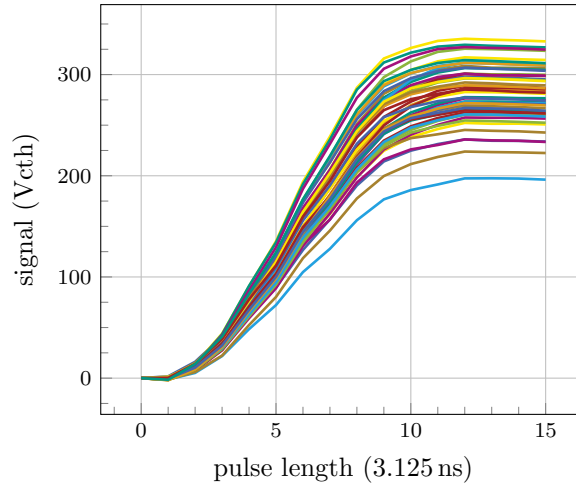
Figure 11.3: Calibration curves for the KARATE injector channels at 2.0 V LED pre-load, latency 90 and DLL 5. The recorded signal for a given pulse lengths varies strongly from channel to channel. For pulse length above 8, the signals saturate for timing reasons.
