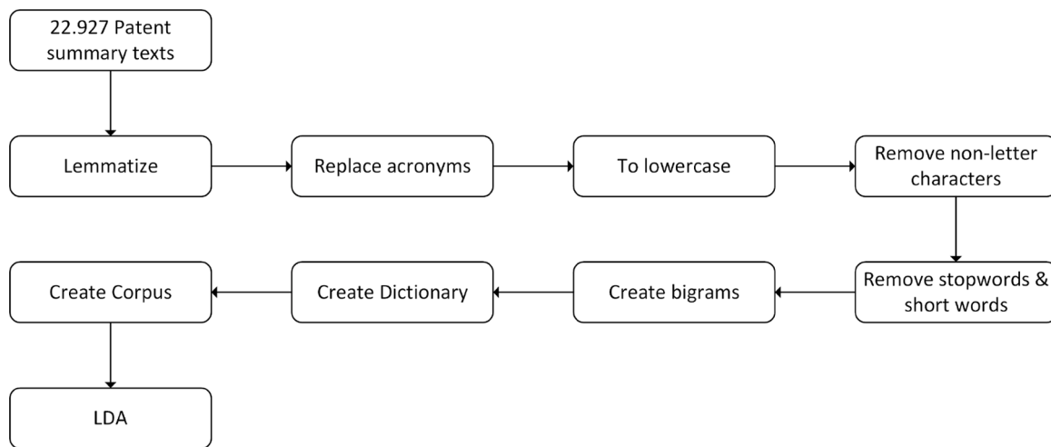
Fig. 4. Data cleaning procedure .
