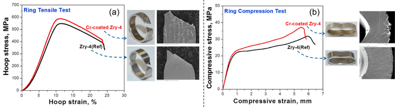
Fig. 24. (a) Ring tensile test results and the picture of the Cr-coated Zr alloy ring after the tensile test. (b) Ring compression test results and the photographs of the Cr-coated Zr alloy ring after the compression test. Reproduced with permission from Ref. [44].
