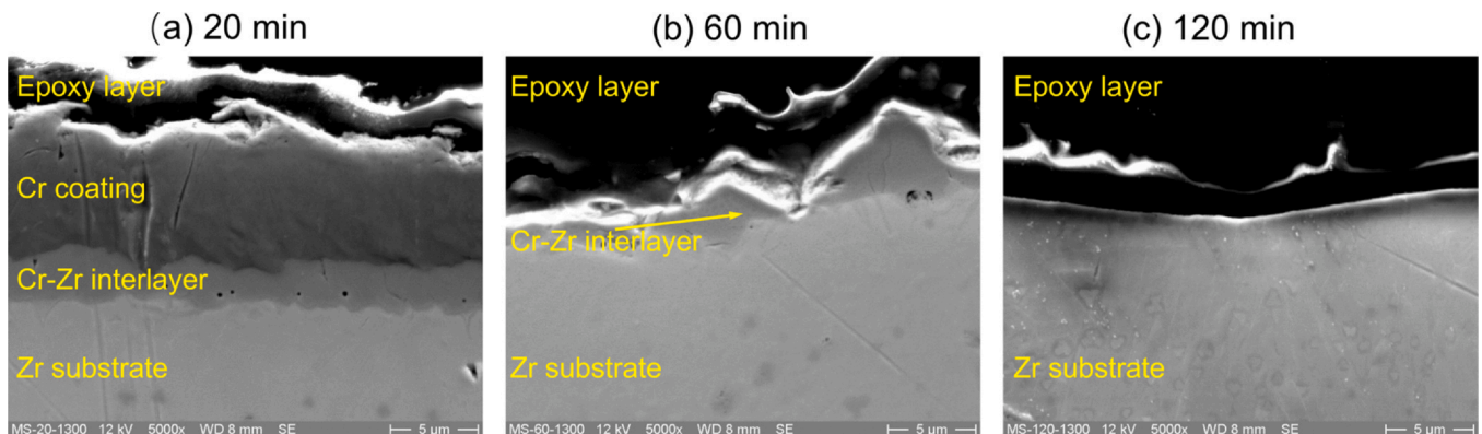
Fig. 15. Evolution of the Cr-Zr interlayer thickness as a function of exposing time at 1300 °C in inert gas environment. Reproduced with permission from Ref. [104].
