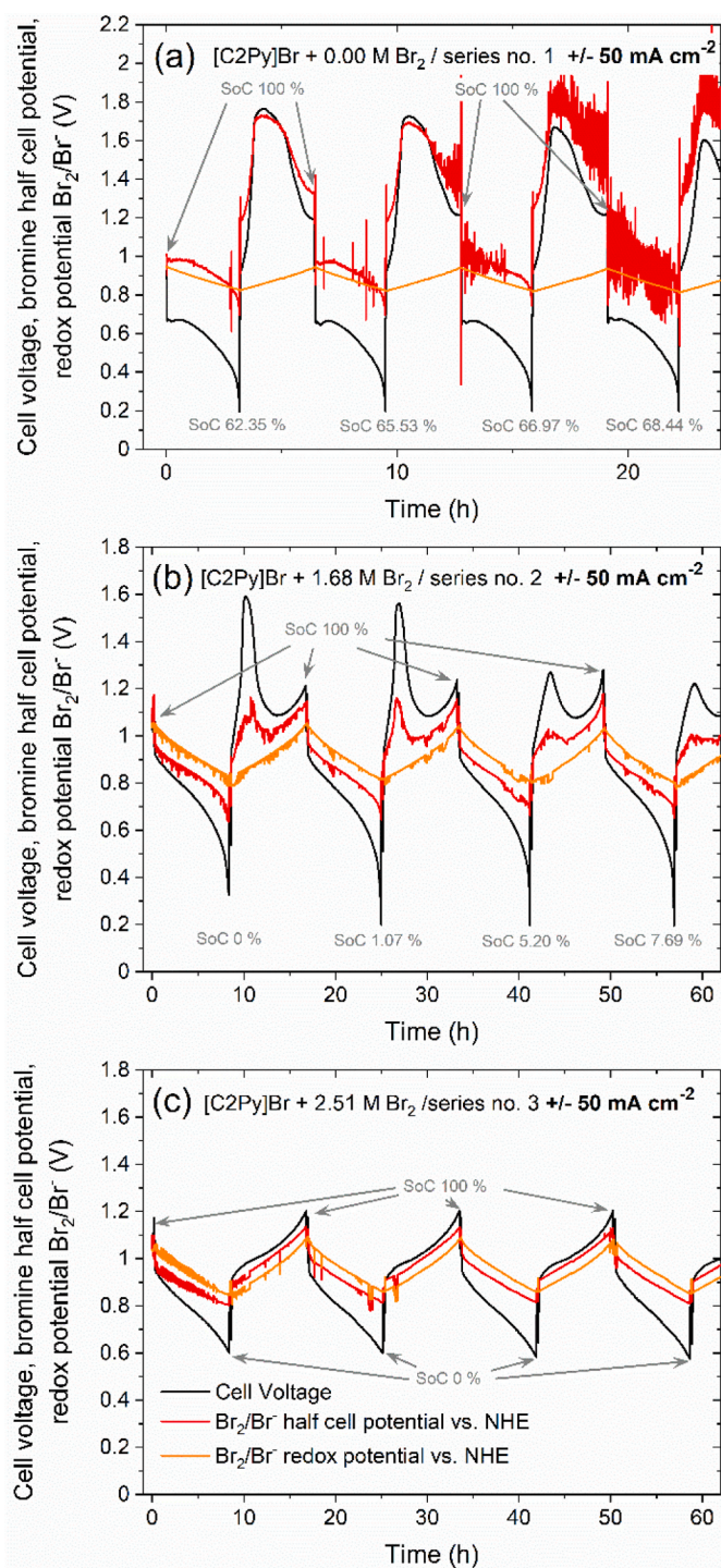
Fig. 6. Cell voltage, positive bromine half cell potential vs. NHE and redox potential of the bromine/bromide electrolyte vs. NHE for electrolyte series (a) no 1 (+0.00 M Br 2 ), (b) no. 2 (+1.68 M Br 2 ) and (c) no. 3 (+2.51 M Br 2 ) for galvanostatic cycling with i = \pm 50 \text{ mA cm}^{-2} in a 40 \text{ cm}^2 H 2 /Br 2 -RFB single cell within thresholds between +3.0 and 0.2 V. In grey letters maximum SoC values before discharge operation and minimum SoC values after discharge operation are shown for the cycling tests in (a–c).
