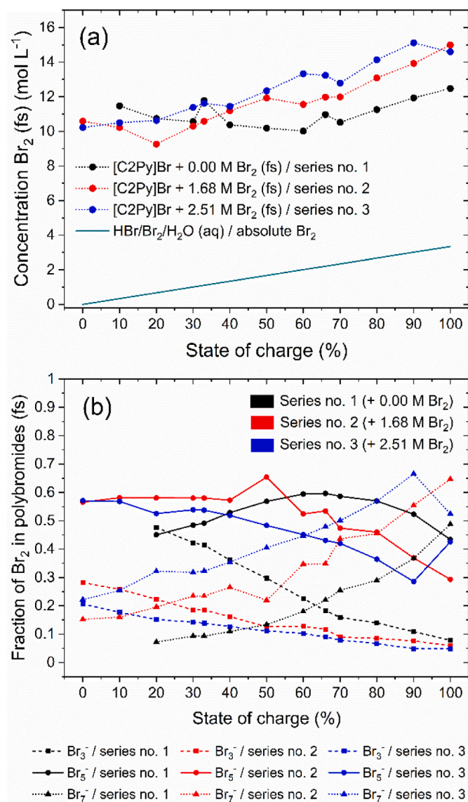
Fig. 4. Br 2 composition in the fused salt: (a) the concentration of Br 2 (fs) and (b) the Br 2 distribution on the polybromides Br 3 - , Br 5 - and Br 7 - , depending on the SoC and on the electrolyte series no. 1 to 3 investigated at \vartheta = 23 \pm 1 °C.
