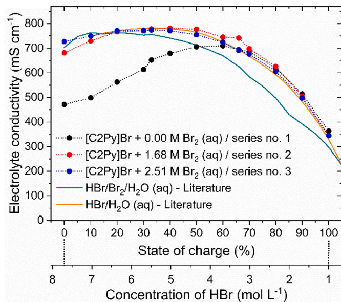
Fig. 5. Electrolyte conductivity of the aqueous electrolyte phase depending on SoC/HBr concentration and electrolyte series (no. 1 - black, no. 2 - red, no. 3 - blue) and conductivity of the BCA-free electrolyte HBr/Br_2/H_2O without an excess of Br_2 (+0.00 M Br_2 ) (green line) from literature [27] (all at \vartheta = 23 \pm 1^\circ C ), as well as comparison with bromine-free and BCA-free, pure HBr/H_2O solutions converted to the SoC scale (orange line) from literature ( \vartheta = 20^\circ C ) [75]. (For interpretation of the references to colour in this figure legend, the reader is referred to the Web version of this article.)
