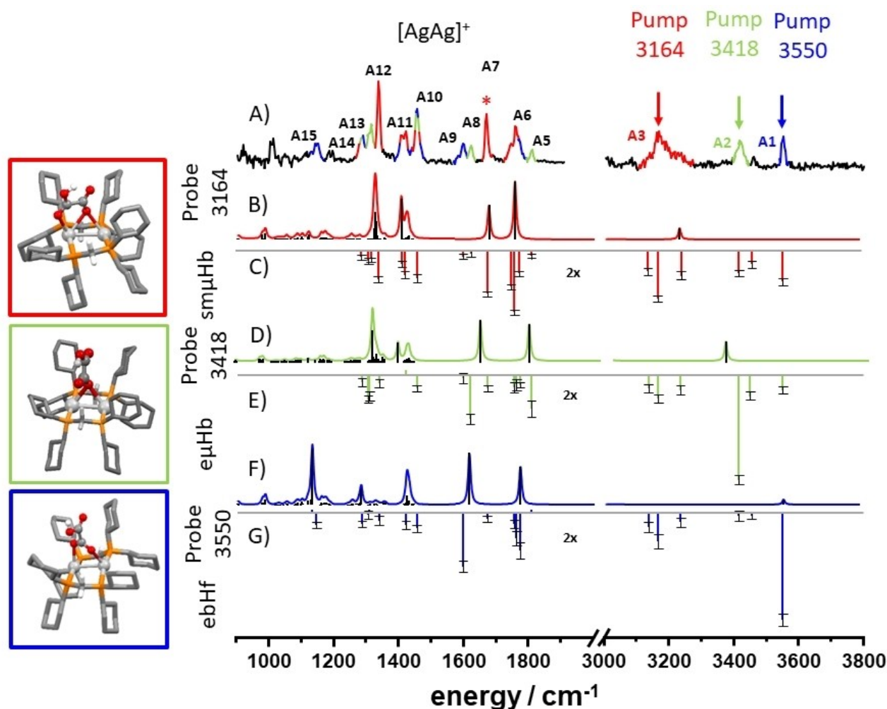
Figure 7. Hydrogen oxalate ( \text{HOx} , \text{HC}_2\text{O}_4^- ) may vary in conformation and coordination when bound to diphosphine stabilized dinuclear [\text{CuCu}]^+ (not shown) and [\text{AgAg}]^+ complexes (left). Isomer sensitive 2cIR-PD pump probe spectroscopy reveals the pump induced attenuation (coloured stick spectra b, d, f) with respect to the 1cIR-PD spectrum (top, a). The attenuations found correlate well with computed DFT spectra (c, e, g) of the presumed isomers. The high amount of IR induced isomerization indicates a considerable fluxionality of HOx when bound in [\text{AgAg}]^+ complexes, in contrast to the revealed stiffness within the [\text{CuCu}]^+ complexes. Reproduced with permission from Ref. [109] Copyright 2021, Wiley-VCH.
