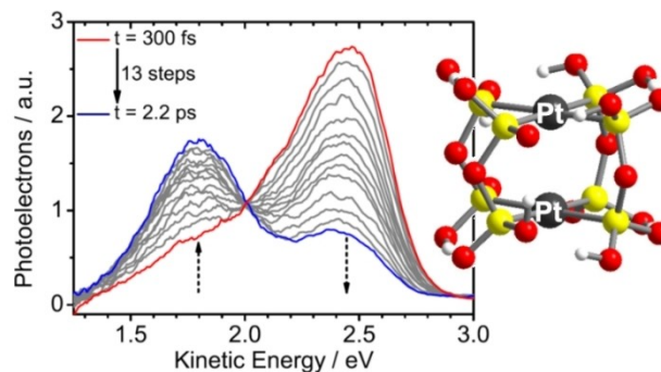
Figure 12. Transient photoelectron spectra and structure of [\text{Pt}_2(\mu\text{-P}_2\text{O}_5\text{H}_2)_4 + 2\text{H}]^{2-} . The isosbestic point and further findings help to identify excited state tunnelling detachment (ESETD) after intersystem crossing (ISC), for further details see text. Modified from Ref. [131], Copyright 2021, Wiley-VCH.
