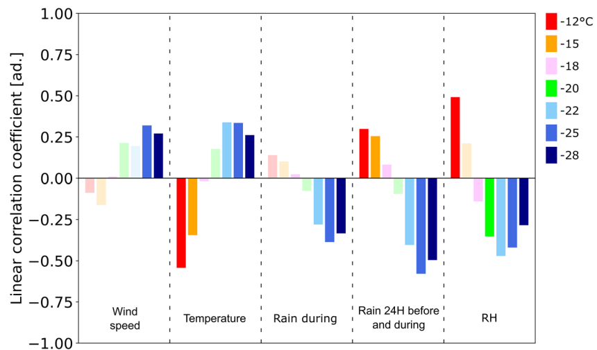
Figure 4. Linear correlation coefficients between the logarithm of the untreated INP concentration and meteorological variables at various processing temperatures. “Rain during” refers to rain occurring during the period of filter sampling, while “rain 24H before and during” refers to rain occurring up to 24 hr before filter sampling as well as during. Pale histogram bars represent non-significant coefficients ( p > 0.05 ).
