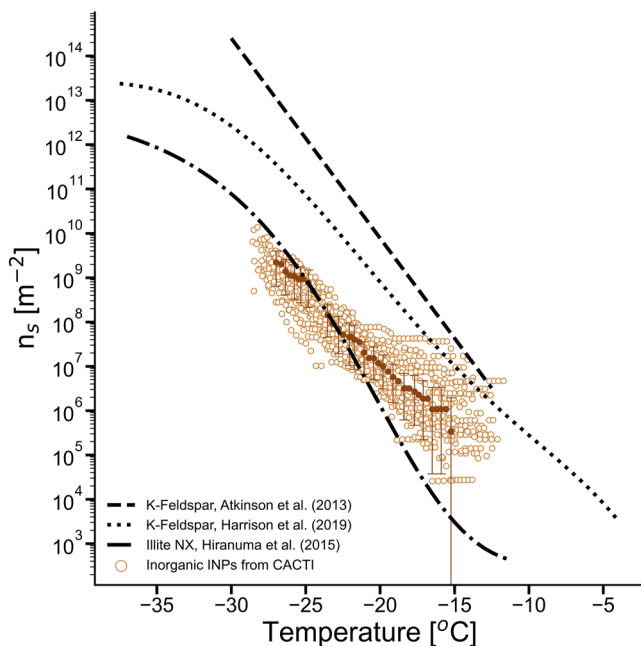
Figure 12. Ice-active surface site density of inorganic INPs measured in this study (brown open circles). Here, n_{\text{INP}} have been normalized using the total surface area of aerosols having a diameter >1.0 \mu\text{m} (see Equation 3). INP parameterizations from Atkinson et al. (2013) and Harrison et al. (2019) were derived from Brunauer-Emmett-Teller (BET) gas adsorption surface measurements while aerosol surface areas in this study were derived by assuming spherical particles (geometric surface), likely underestimating the real surface area of the particles. Hence, the K-feldspar parameterizations were converted to estimated geometric surface area parameterizations, applying the conversion factor 2.6/0.89 used in DeMott et al. (2018) and derived from the K-feldspar sample used in their study. For clarity, the uncertainties in n_s are shown for one sample (11 November 2018) only. On that day, surface areas were derived from nephelometer measurements, hence resulting in higher uncertainties in n_s compared to surface areas derived from SMPS-UHSAS-APS (see Supporting Information S1).
