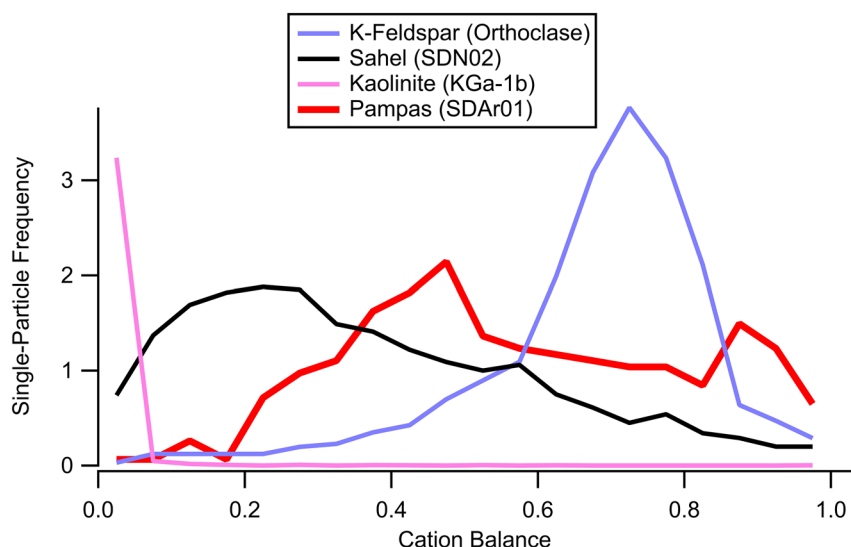
Figure 9. Cation balance ( K + Na/Al + Si ) of 325 single soil particles of SDAr01 by LAAPTOF single-particle mass spectrometry reveals it was somewhat higher than pure kaolinite, but lower than pure K-feldspar.
