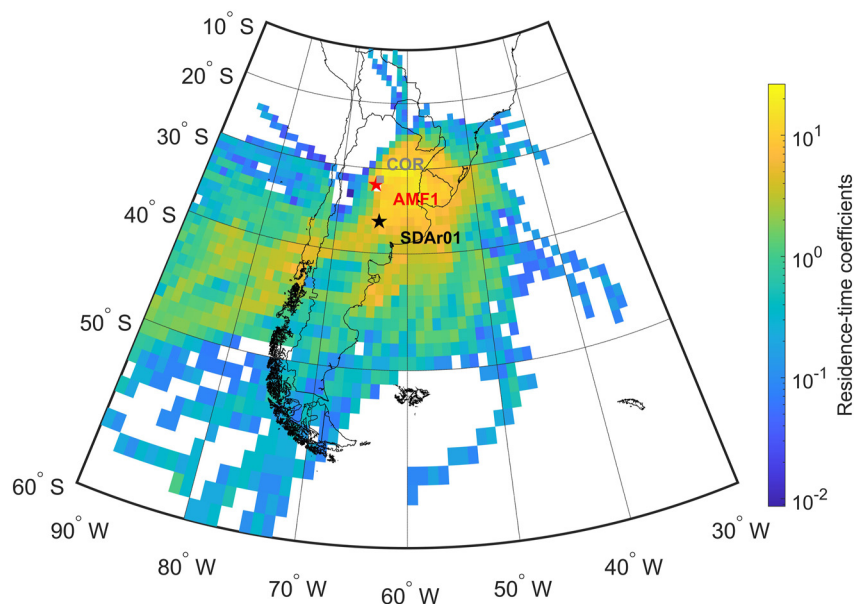
Figure 1. Residence-time-weighted 5-day back-trajectories for the period of the campaign. The coefficients of the grid cells encompass, and are weighted by, the time the air mass spent in the cells before arriving at AMF1 (red star on the map) and the distance between the cells and AMF1. Cells with the strongest coefficients indicate likely principal sources of the particles observed at AMF1. The sampling location of the SDAr01 sample is indicated by the black star and the city of Córdoba by the gray square.
