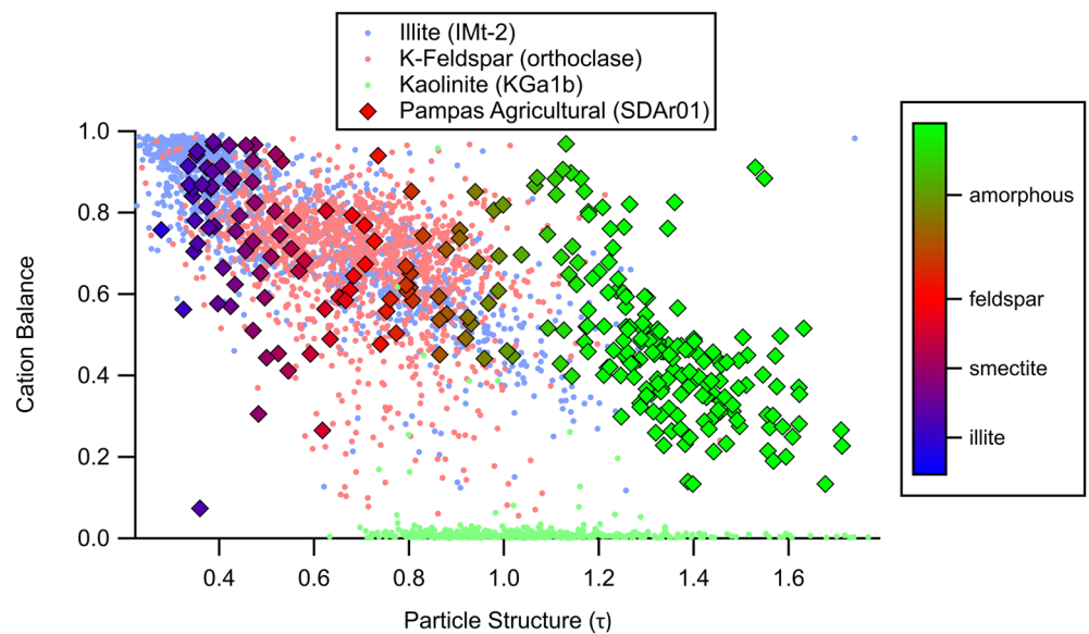
Figure 10. Cation balance versus crystal structure analysis ratio ( \tau ) of 286 particles in pampas agricultural soil sample SDAr01 (larger diamonds, with black outlines) by LAAPTOF single-particle mass spectrometry. The color scale is our interpretation of particle mineralogy based on comparison with pure mineral proxies (colored dots), illite (IMt-2) and Kaolinite (KGa1b) from the clay mineral society, and K-feldspar from a crushed crystal of orthoclase.
