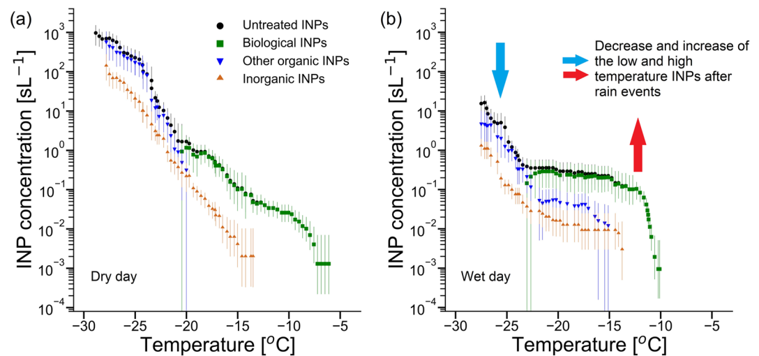
Figure 5. INP spectra for (a) A “dry” day (17 November 2018), that is, with no rain occurring 24 h before and during the period of sampling, and (b) A “wet” day (12 November 2018) with RH > 80% and precipitation occurring within 24 h before and/or during sampling (on this day, rain occurred 6 h before and during sampling). The effect of rain upon INP populations is generalized by the arrows. Error bars indicate 95% confidence intervals.
