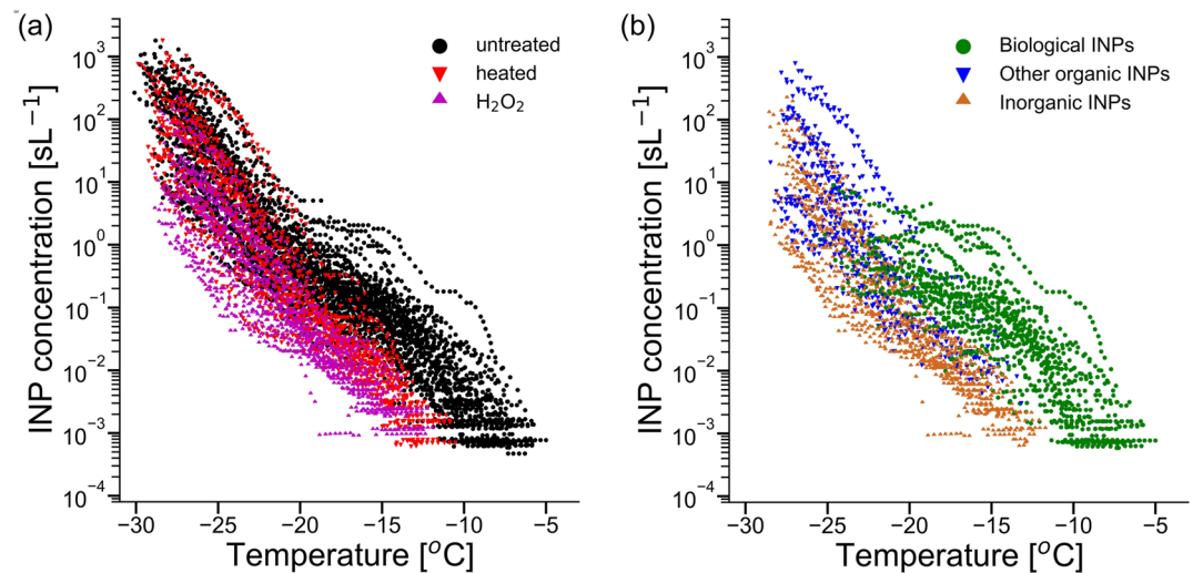
Figure 3. Ice nucleation activation temperature spectra of processed INP samples. (a) INP spectra of untreated samples superimposed over INP spectra following heat and \text{H}_2\text{O}_2 treatments. (b) Spectra of computed biological, other organic and inorganic INP contributions derived from statistically significant differences between the untreated and heated spectra, significant differences between the heat-treated and the \text{H}_2\text{O}_2 -digested spectra, and the residual activity remaining after \text{H}_2\text{O}_2 oxidation (see Section 2.3). Uncertainties are omitted here for clarity, but are shown in Figure 2a.
