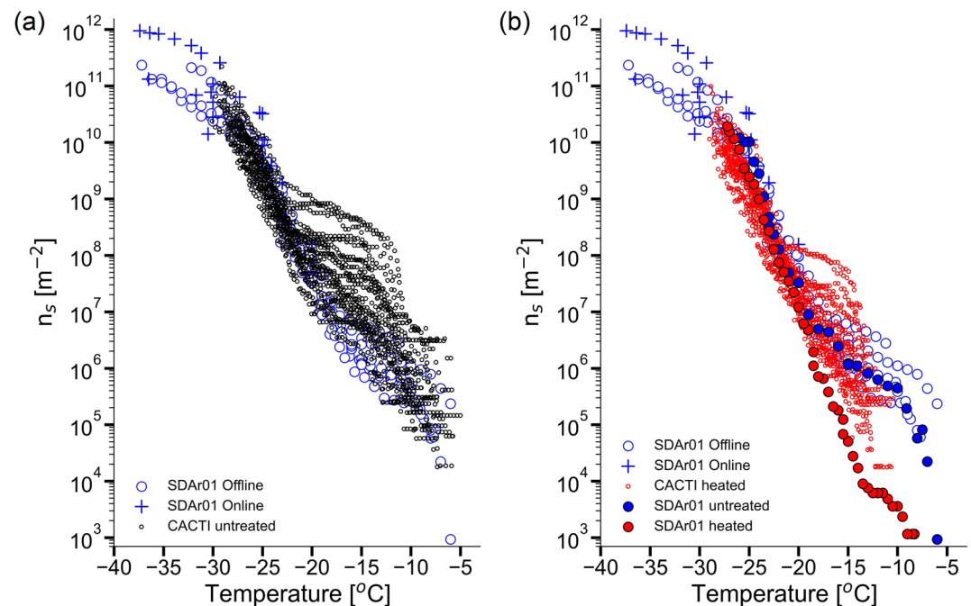
Figure 13. Surface site density of SDAr01 samples from the FIN-02 campaign (DeMott et al., 2018) plotted alongside the surface site density of (a) The untreated INP spectra from this study, and (b) The heat treated INPs from this study. The black outlined blue and red dots represent values of the untreated and heated SDAr01 sample.
