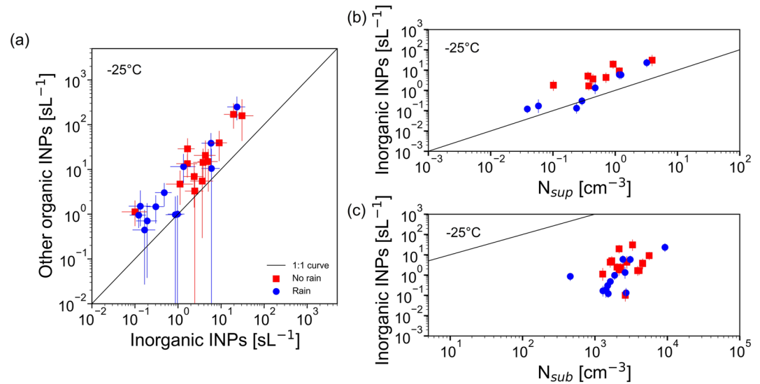
Figure 8. (a) Concentration of other organic INPs vs. inorganic INPs active at -25^{\circ}\text{C} during days with and without rain. (b) Concentration of inorganic INPs active at -25^{\circ}\text{C} versus concentration of supermicron particles ( N_{\text{sup}} ), and (c) Concentration of submicron particles ( N_{\text{sub}} ). Panel (a) shares its legend with panels (b) and (c). Lines show 1:1 relationships.
