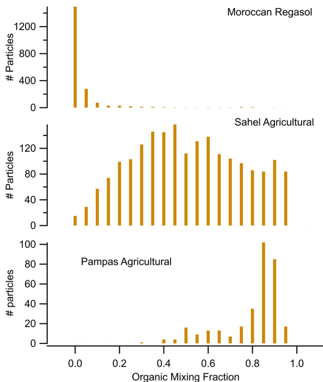
Figure 11. Internal mixing state of aerosolized soil samples analyzed by single-particle mass spectrometry. Organic mixing fraction is calculated from the CNO/(CNO + SO_4 + Cl) sub-composition analysis of negative ion marker peaks.
