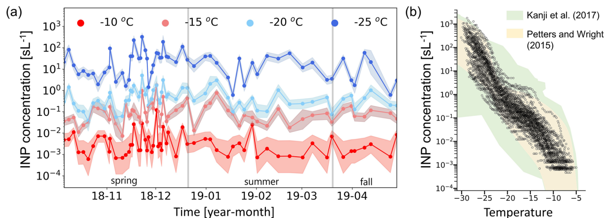
Figure 2. (a) Ice nucleating particle concentrations at the AMF1 site during the campaign, at four processing temperatures. The shaded area enclosing each represents the 95% confidence intervals. (b) INP spectra of all samples (error bars omitted for clarity). The light green shaded area represents upper and lower limits of global field INP concentration measurements summarized in Kanji et al. (2017, Figures 1–10), while the yellow shaded area represents atmospheric INP concentration ranges estimated from precipitation samples collected in North America, Europe and Antarctica (Petters & Wright, 2015).
