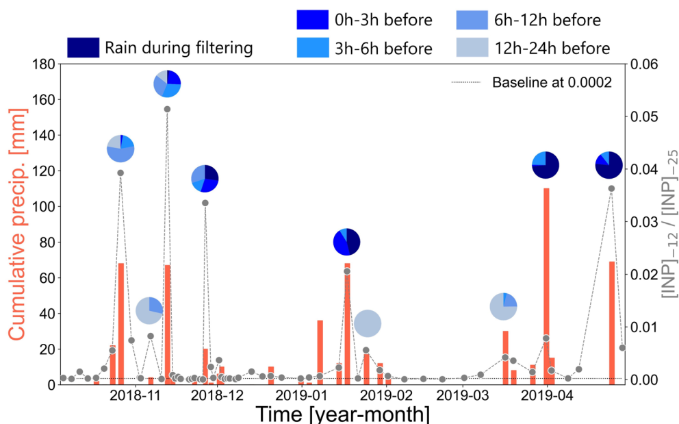
Figure 6. Time series of the ratio of [INP]_{-12^{\circ}C}/[INP]_{-25^{\circ}C} (i.e., ratio of concentrations of INPs active at -12^{\circ}C with INPs active at -25^{\circ}C ). Each point represents one INP sample (the dashed gray lines linked the dots for guiding the eye). Total precipitation within 24 h before and during filter sampling is given by the bars, while the proportions of rain occurring within different timespans are shown by the pie charts. The baseline for dry sampling days is indicated by the dotted line.
