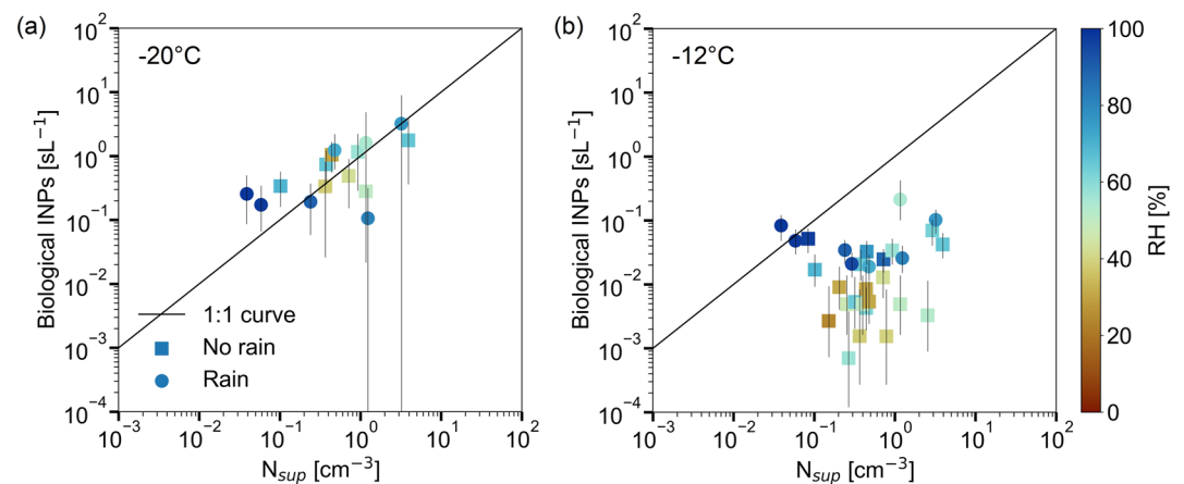
Figure 7. The concentration of biological INPs active at (a) -20^{\circ}\text{C} and (b) The concentrations of all INPs (likely all biological) active at -12^{\circ}\text{C} , versus the concentrations of aerosol particles with a diameter >1\ \mu\text{m} ( N_{\text{sup}} ). Circles correspond to filters sampled during rainy days (rain up to 12 h before sampling), while squares indicate non-rainy days. The average relative humidity during sampling is given by the color. Error bars indicate 95% confidence intervals. Lines show 1:1 relationships.
