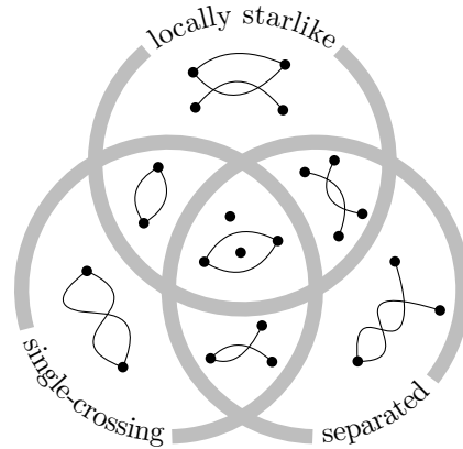
Figure 1: Illustrating some drawing styles of topological multigraphs. A branching drawing is separated, single-crossing and locally starlike.
