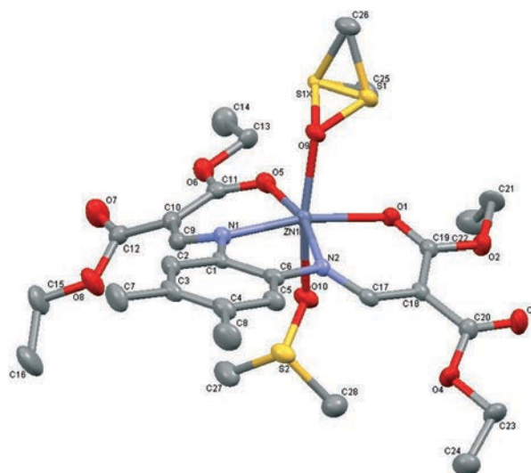
Fig. 5 Displacement ellipsoid plot of Zn[ 3b ] [Zn( 3b )(DMSO) 2 ].
