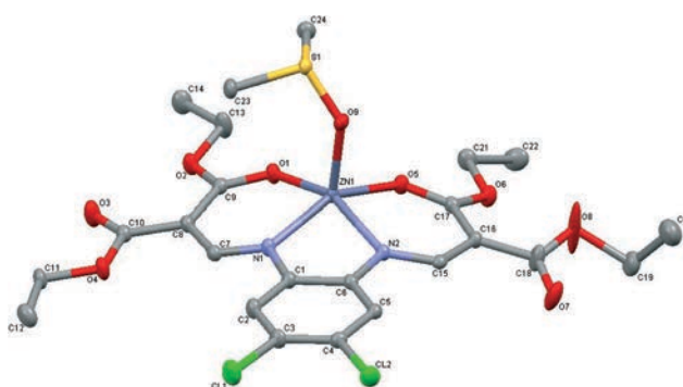
Fig. 4 Displacement ellipsoid plot of Zn[ 2b ] [Zn( 2b )(DMSO)].
