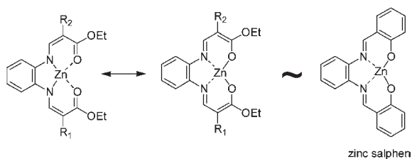
Scheme 4 Mesomeric forms of the Zn \text{N}_2\text{O}_2 structure and analogy with zinc salphens.
