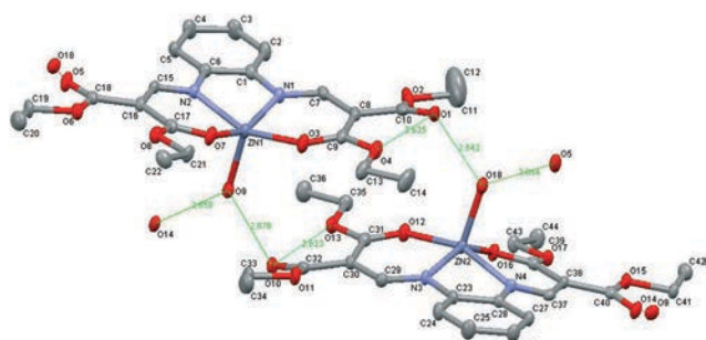
Fig. 3 Displacement ellipsoid plot of Zn[ 1b ] [Zn( 1b )(H 2 O)] 2 showing the two independent molecules.
