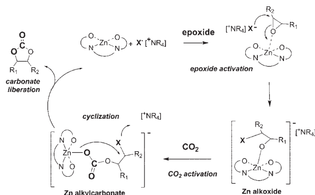
Scheme 5 Mechanism proposed for the zinc \text{N}_2\text{O}_2 /NBu 4 I catalytic system.
