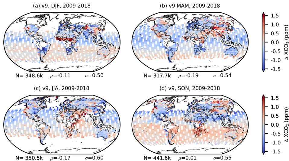
Figure 11. Seasonal maps of the mean \Delta XCO_2^{MMM} (GOSAT – MMM) spanning 2009 through 2018 for DJF (a), MAM (b), JJA (c), and SON (d) at 2.5° latitude by 5° longitude resolution. Grid boxes containing fewer than 10 collocations are colored white.
