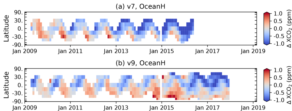
Figure 12. Time series of \Delta XCO_2^{MMM} (ACOS GOSAT v9 – MMM) versus latitude at 30 d by 15° resolution for ocean H-gain observations for v7.3 (a) and v9 (b). Grid cells containing fewer than 10 collocations are colored white.
