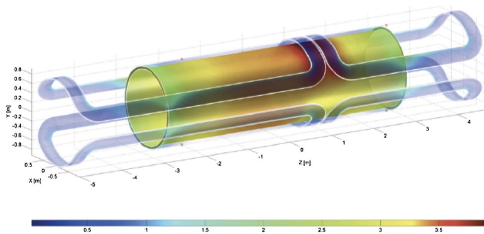
Figure 220. The coil arrangement of the solenoid and dipole systems housed in a common cryostat. Reproduced from [1]. © IOP Publishing Ltd. CC BY 3.0
