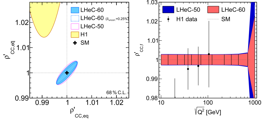
Figure 65. Left: anomalous modifications of the CC form factors \rho'_{CC,eq} and \rho'_{CC,eq\bar{q}} for different LHeC scenarios in comparison with the H1 measurements [423]. Right: scale-dependent measurement of the anomalous modification of the CC form factor \rho'_{CC}(Q^2) , assuming \rho'_{CC,eq} = \rho'_{CC,eq\bar{q}} = \rho'_{CC} .
