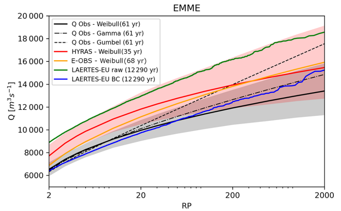
Figure 7. Return values of observed and simulated discharges Q at EMME station. Given are the Weibull (solid black), Gumbel (dashed black), and gamma (dot-dashed black) distributions for observed discharges as well as the Weibull distributions for the simulation forced with observed precipitation from E-OBS (orange) and HYRAS (red). The results from uncorrected LAERTES-EU-driven simulations are given in green, and those driven by corrected LAERTES-EU data are shown in blue. The shaded areas represent the 95 % confidence intervals of HYRAS (red) and Q Obs-Weibull (gray). The length of each time series is given in the legend.
