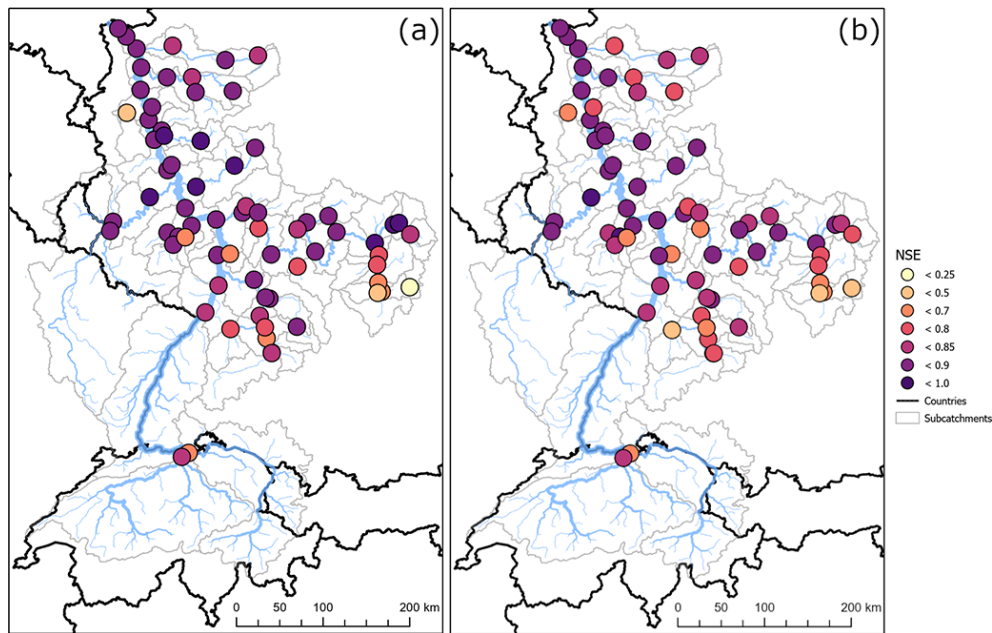
Figure 5. Nash–Sutcliffe model efficiency coefficient (NSE) for the 71 catchments of the Rhine basin (validation period 1986–2009) with (a) HYRAS and (b) E-OBS as HM forcing. Higher values indicate better agreement.
