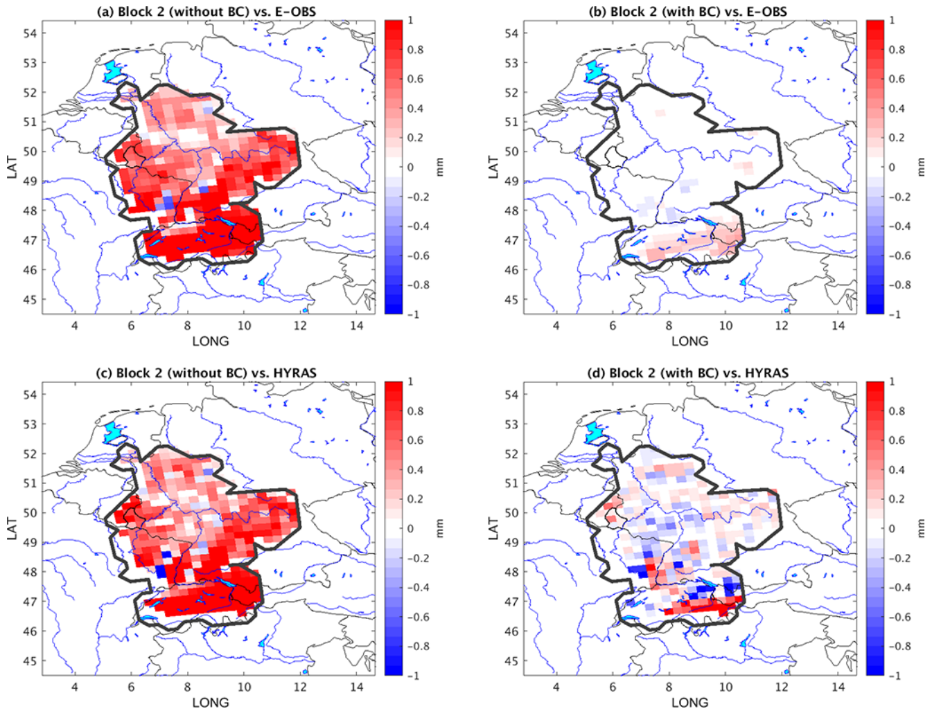
Figure 2. Bias within the Rhine basin (bold black contour) of daily precipitation [in mm] for the LAERTES-EU ensemble mean based on data block 2 (a) towards E-OBS uncorrected, (b) towards E-OBS after bias correction, (c) towards HYRAS uncorrected, and (d) towards HYRAS after bias correction. Thin black lines show country borders; blue lines indicate rivers; cyan-shaded areas show lakes.
