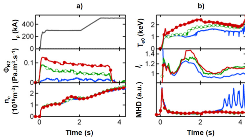
Figure 8. Example of 3 consecutive pulses, #54762 (blue), #54764 (green), #54765 (red), with increasing nitrogen seeding rate. (a) Plasma current, identical for the 3 pulses (top), nitrogen injection rate (middle) and volume-averaged plasma density (bottom); (b): central electron temperature, internal inductance and MHD level.
