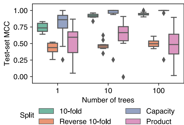
(a) Prediction performance for random forests.
