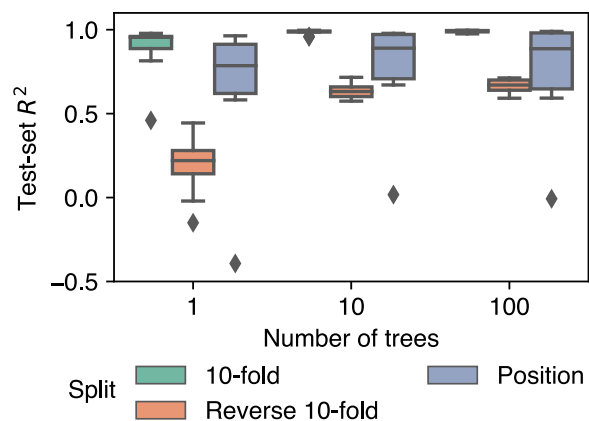
(a) Prediction performance for random forests.
