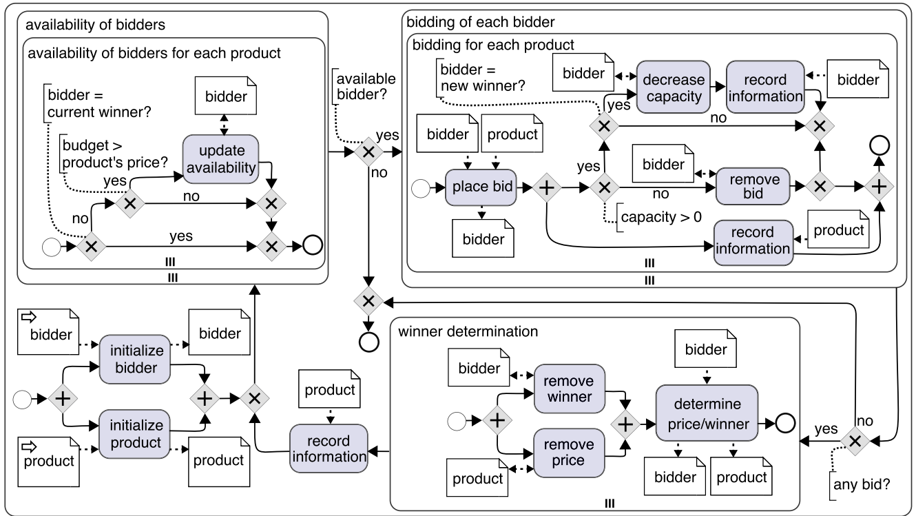
FIGURE 2. Simplified process model of an SMR auction in BPMN notation.
