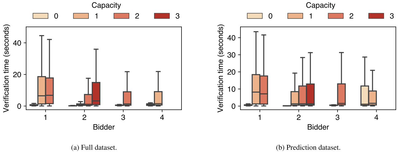
FIGURE 3. Distribution of verification time (excluding outlier points) for different capacities of individual bidders.
