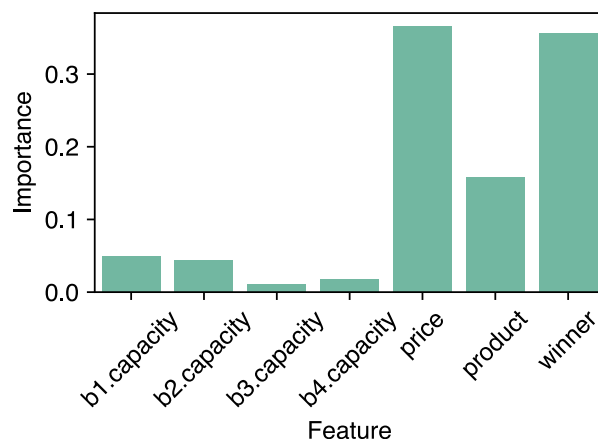
(b) Average feature importance for random forests with 100 trees in 10-fold cross-validation.
