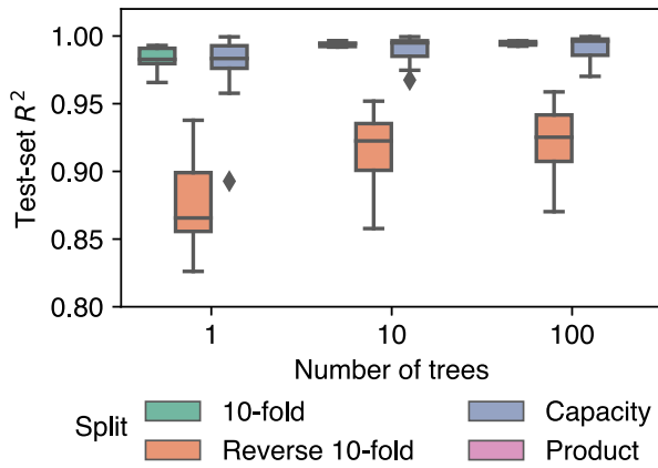
(a) Prediction performance for random forests. Y-axis truncated for readability, thus no results for product-based split.
