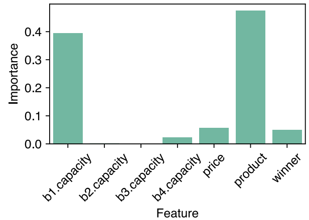
(b) Average feature importance for random forests with 100 trees in 10-fold cross-validation.
