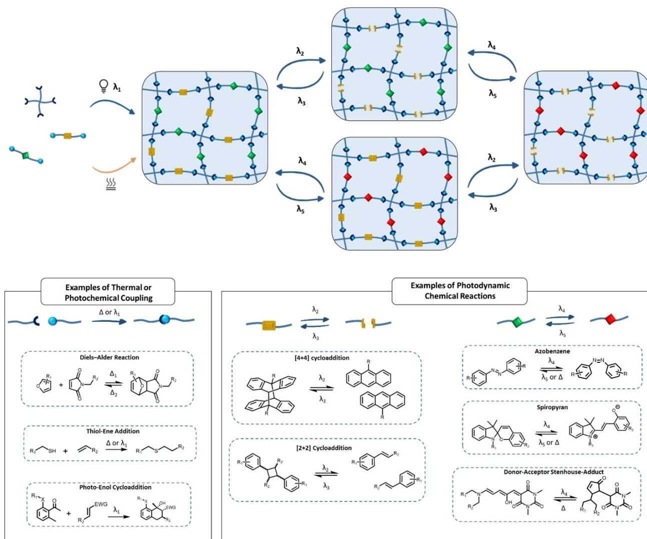
Figure 1. Conceptual scheme (top) of photodynamic networks that can be formed via thermal- or light-induced crosslinking, during which photoreversible chromophores are incorporated within the networks, enabling switching of chemical and physical properties of the resultant networks by highly specific wavelengths of light. Examples (bottom) of chemical reactions, including chemical coupling (left) and reversible photochemical transformations (right), which can be employed in the top scheme.
