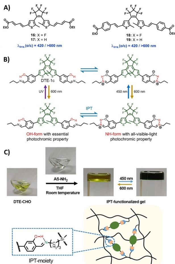
Figure 6. A) Representative chemical structures of red-shifted diarylethenes' \pi -conjugation at the 5,5'-positions; reproduced with permission from Ref. [31b] Copyright (2020) Elsevier. B) Fully visible light photochromism of diarylethene via IPT, and C) formation of a photoresponsive crosslinked structure containing the red-shifted diarylethene (AS-NH 2 : amino-functionalised siloxane polymer). Reproduced with permission from Ref. [32] Copyright (2019) American Chemical Society.
