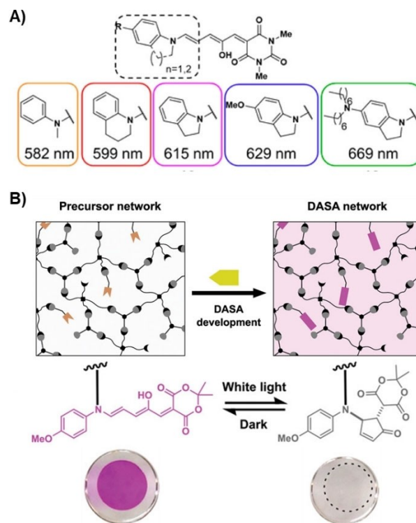
Figure 7. A) Representative structures of red-shifted DASAs with absorbance extending well into the NIR region; reproduced with permission from Ref. [34b] Copyright (2019) American Chemical Society. B) Design of a DASA-incorporated polymer network and schematic depiction of the photoisomerization, enabling the change in material colour. [35]
