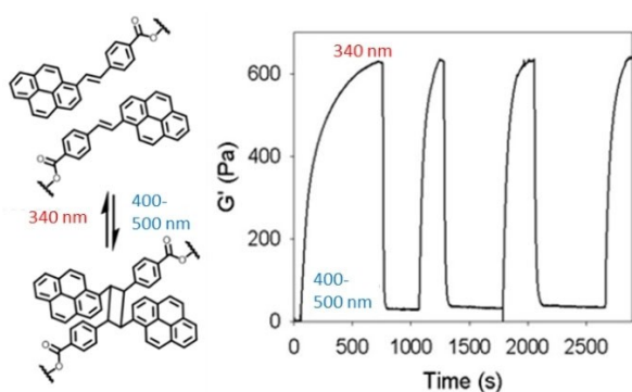
Figure 2. Reversible [2 + 2] photocycloaddition of red-shifted styrylpyrene and its application in the wavelength-orthogonal crosslinking and degradation of a PEG hydrogel, followed by photorheological assessment. Reproduced with permission from Ref. [10]. Copyright (2018) American Chemical Society.
