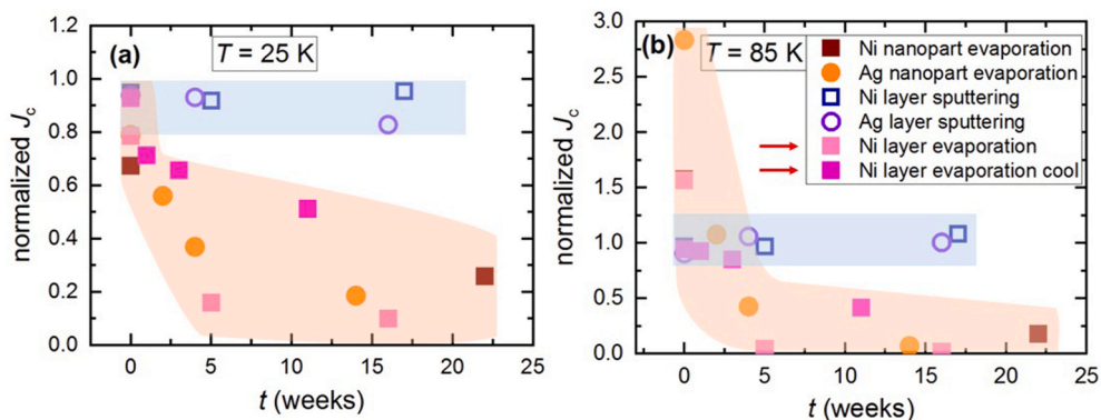
Fig. 4. Time evolution of the normalized J_c at 25 K and 85 K extracted from hysteresis loops. Light and dark pink symbols refer to continuous thin films prepared by regular evaporation, one at room temperature and one cooled with LN2, to investigate the effect of microstructure of the metallic film and the temperature during deposition. (For interpretation of the references to color in this figure legend, the reader is referred to the Web version of this article.)
