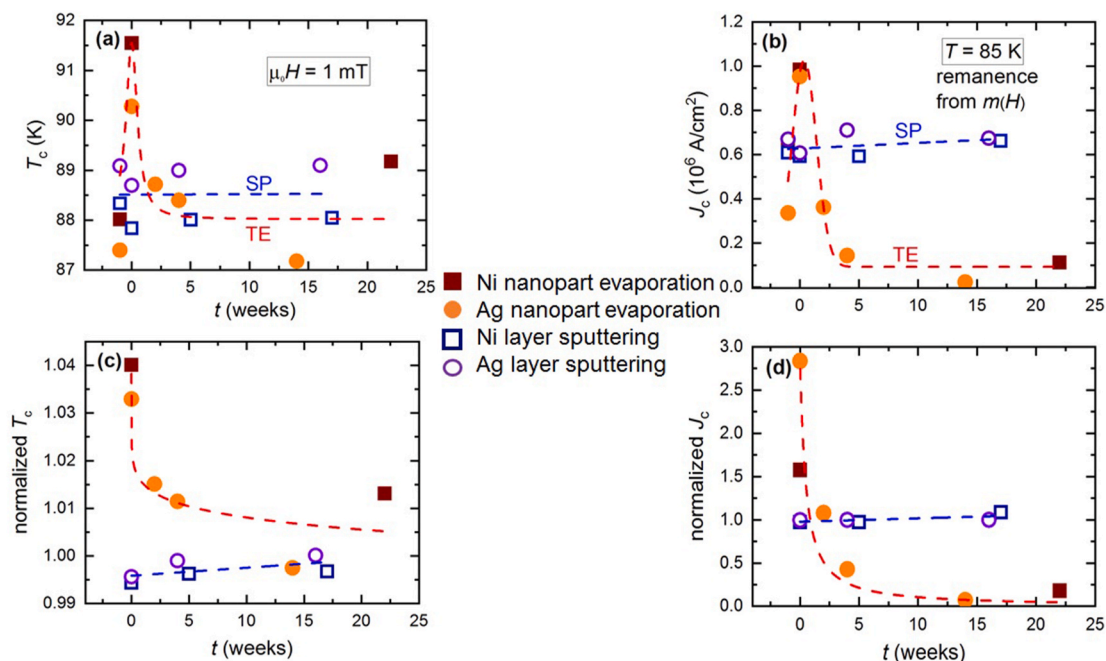
Fig. 3. a) Time evolution of T_c , the first points correspond to the initial measurements of pristine YBCO samples, 0 marks the measurement after deposition of Ni or Ag and the other values refer to measurements after several weeks. b) J_c at 85 K extracted from the hysteresis curves in remanent state. c) and d) depict a different representation of a) and b) where the data are normalized to the initial values before deposition, M is Ag or Ni. Dashed lines are guide to the eyes. Blue refers to sputtered metals, red to evaporated ones. (For interpretation of the references to color in this figure legend, the reader is referred to the Web version of this article.)
