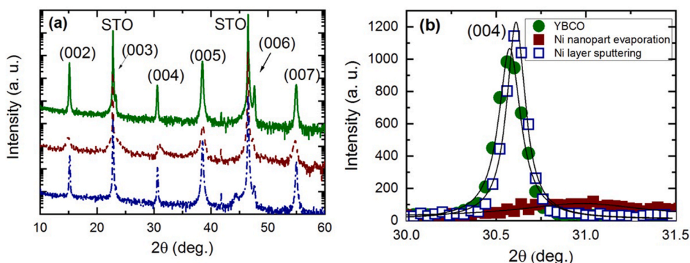
Fig. 5. a) XRD pattern for a YBCO film (green), YBCO/Ni nanoparticles prepared by glancing angle evaporation (brown) after 22 weeks and YBCO/Ni layer deposited using sputtering (blue) after 17 weeks b) Magnification of the (004) peak. (For interpretation of the references to color in this figure legend, the reader is referred to the Web version of this article.)
