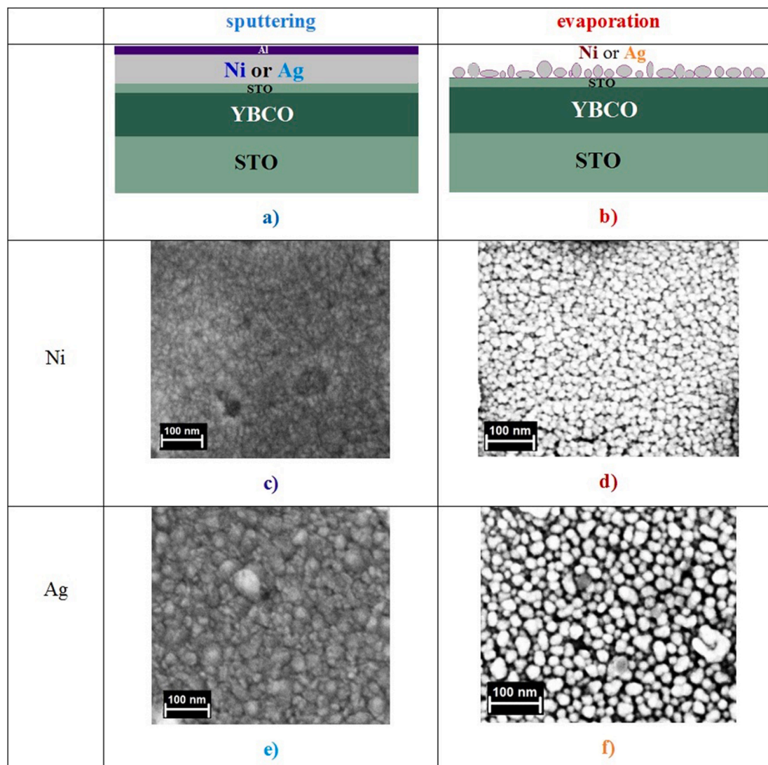
Fig. 1. Sketch of the sample stack for sputtered (a) and evaporated (b) metals; SEM images of the surface for (c) Ni layer, (d) Ni nanoparticles, (e) Ag layer and (f) Ag nanoparticles.
